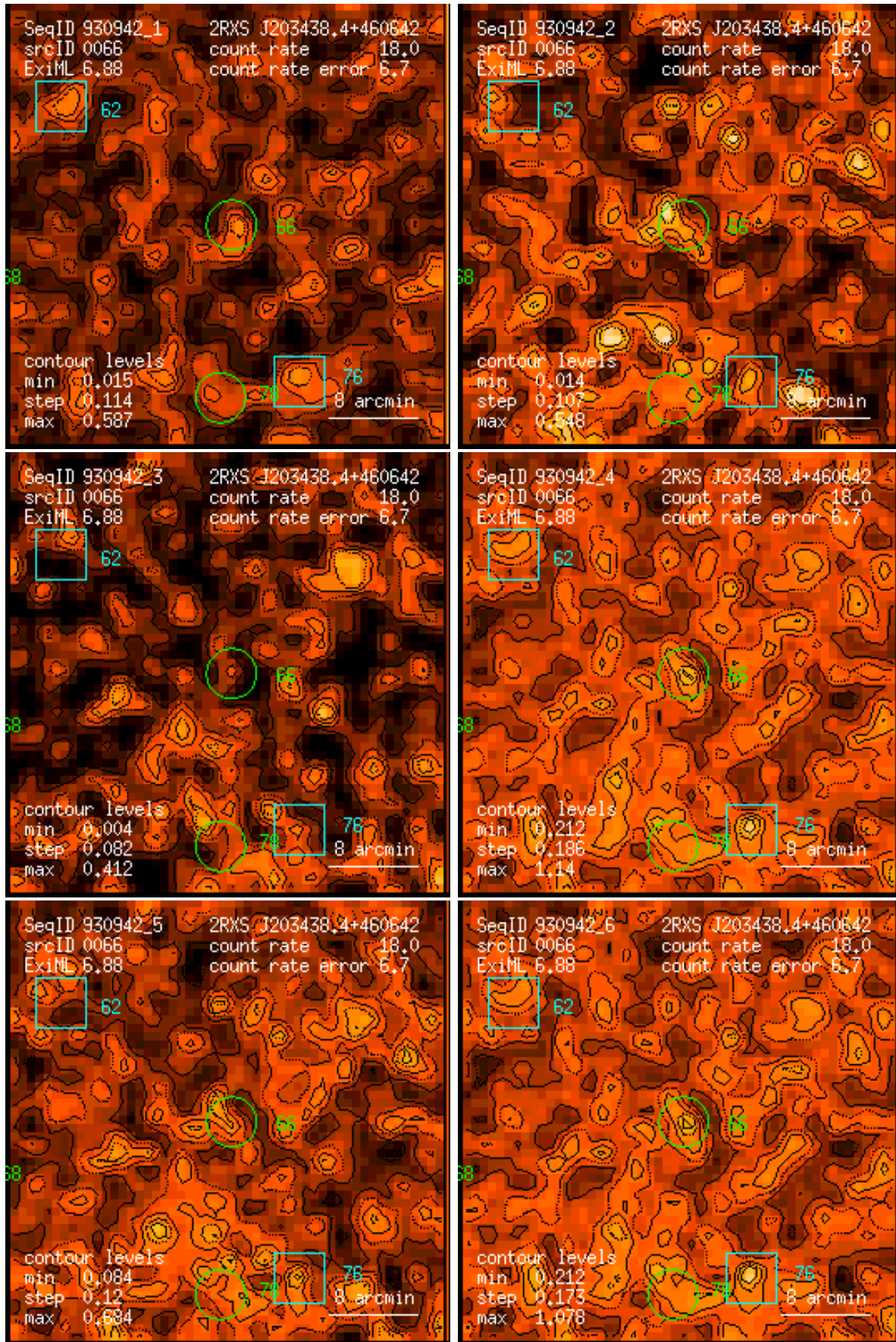
Figure 66: RASS 930942: detection 0066: band rate images, Gaussian filter: (1) PSPC channels 11 – 41, (2) 52 – 90, (3) 91 – 201, (4) 11 – 235, (5) 52 – 201, (6) 11 – 201. Broad band rates in counts/ks. Band rate contour levels in counts/ks/arcmin 2 .
