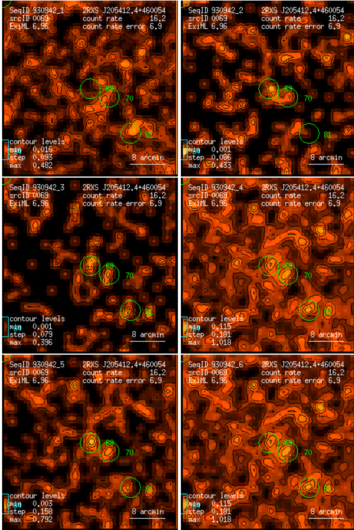
Figure 69: RASS 930942: detection 0069: band rate images, Gaussian filter: (1) PSPC channels 11 – 41, (2) 52 – 90, (3) 91 – 201, (4) 11 – 235, (5) 52 – 201, (6) 11 – 201. Broad band rates in counts/ks. Band rate contour levels in counts/ks/arcmin 2 .
