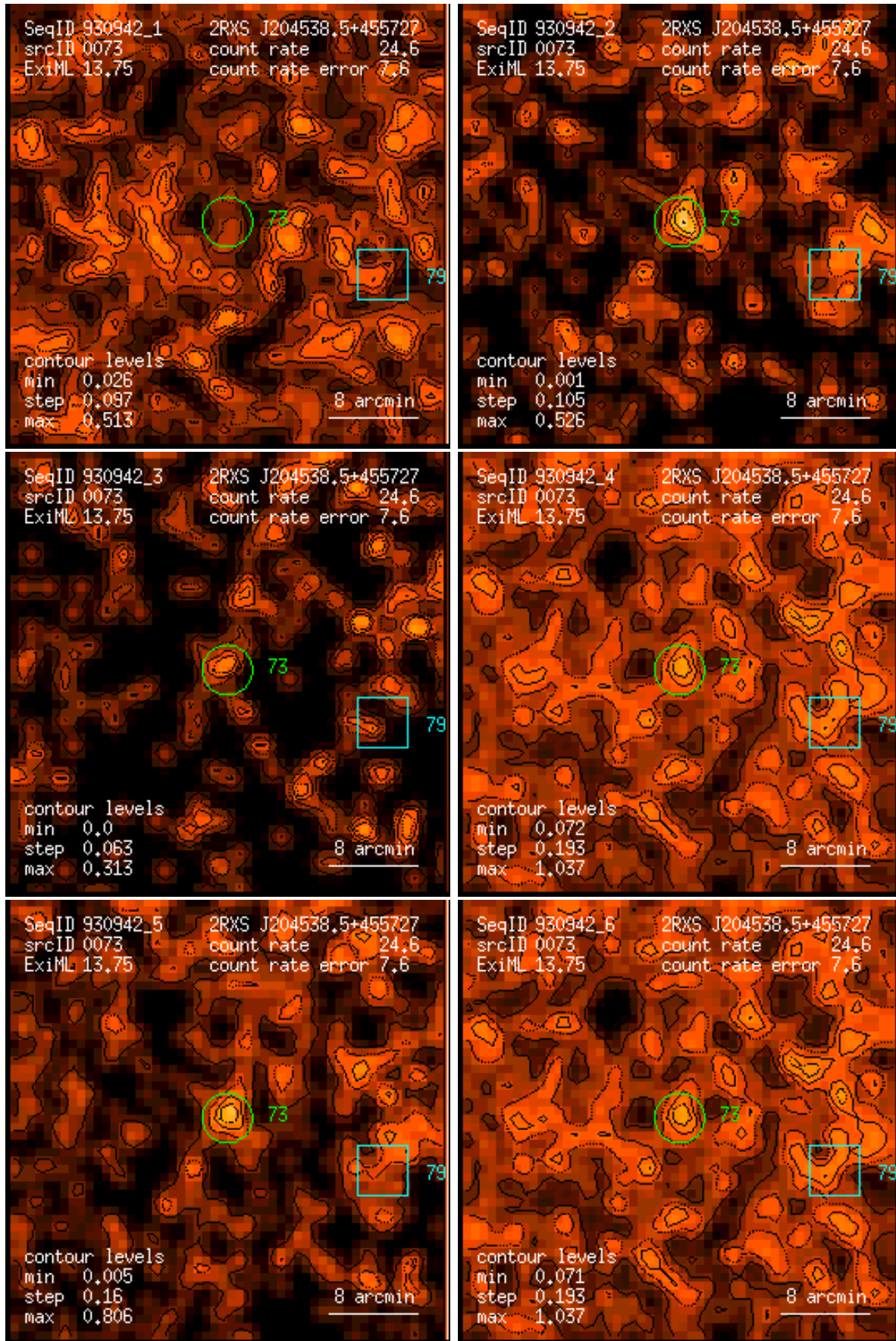
Figure 73: RASS 930942: detection 0073: band rate images, Gaussian filter: (1) PSPC channels 11 – 41, (2) 52 – 90, (3) 91 – 201, (4) 11 – 235, (5) 52 – 201, (6) 11 – 201. Broad band rates in counts/ks. Band rate contour levels in counts/ks/arcmin 2 .
