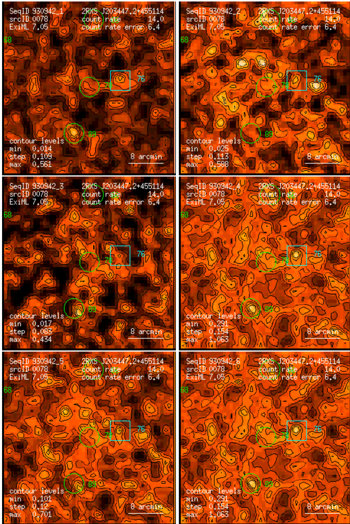
Figure 78: RASS 930942: detection 0078: band rate images, Gaussian filter: (1) PSPC channels 11 – 41, (2) 52 – 90, (3) 91 – 201, (4) 11 – 235, (5) 52 – 201, (6) 11 – 201. Broad band rates in counts/ks. Band rate contour levels in counts/ks/arcmin 2 .
