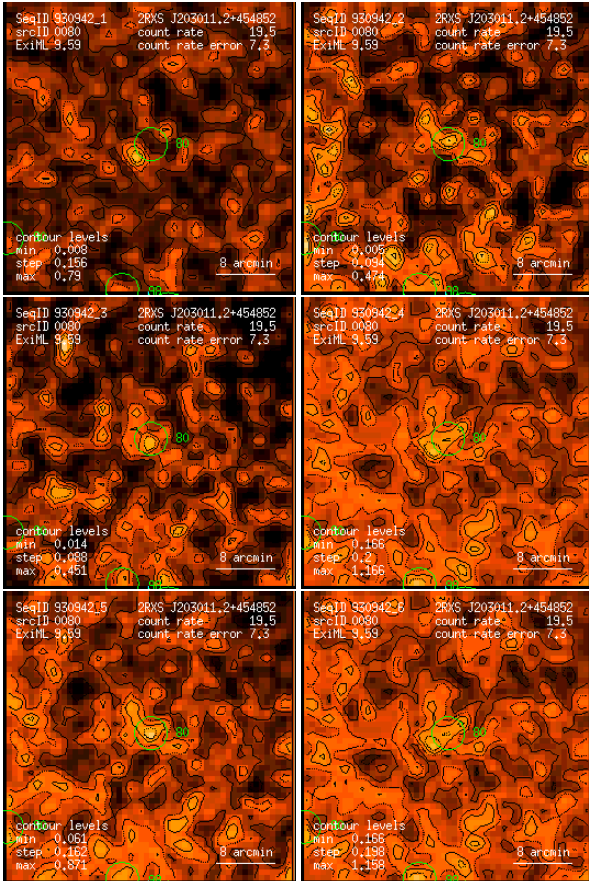
Figure 80: RASS 930942: detection 0080: band rate images, Gaussian filter: (1) PSPC channels 11 – 41, (2) 52 – 90, (3) 91 – 201, (4) 11 – 235, (5) 52 – 201, (6) 11 – 201. Broad band rates in counts/ks. Band rate contour levels in counts/ks/arcmin 2 .
