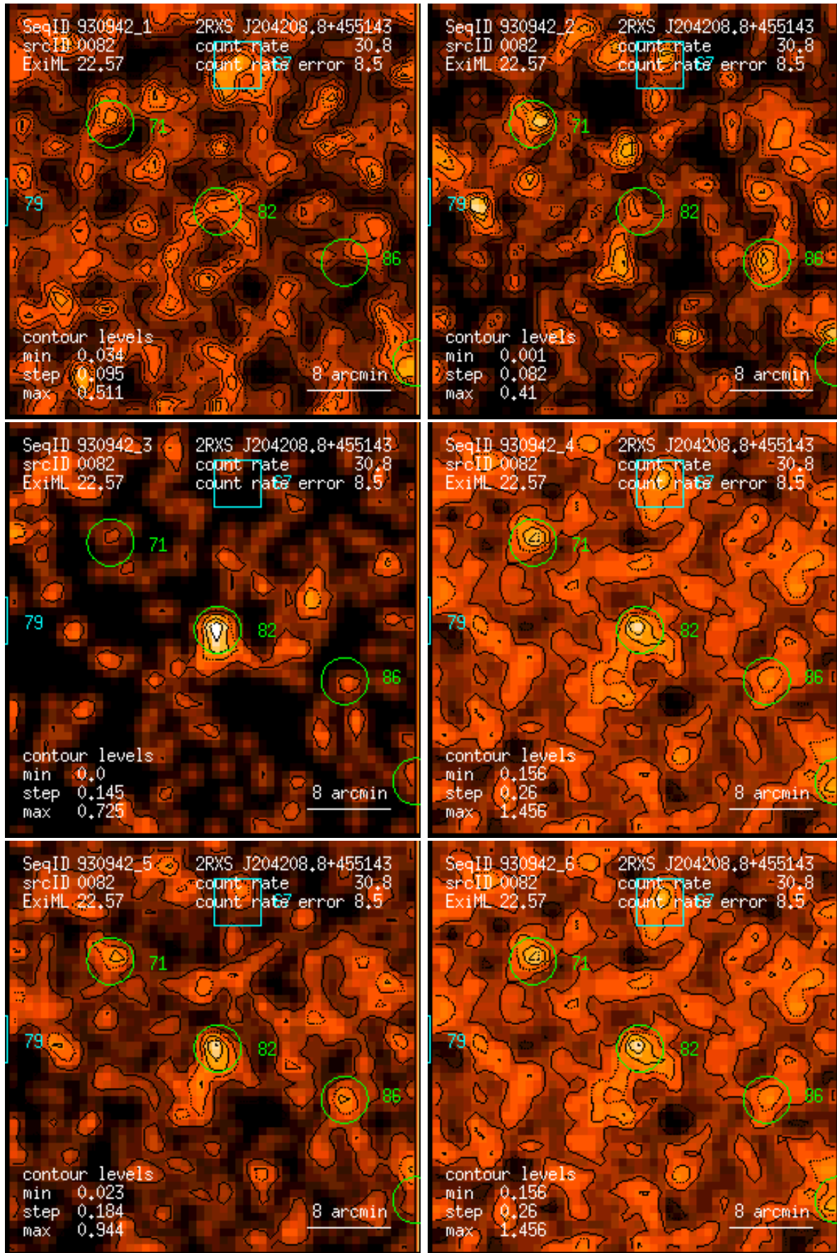
Figure 82: RASS 930942: detection 0082: band rate images, Gaussian filter: (1) PSPC channels 11 – 41, (2) 52 – 90, (3) 91 – 201, (4) 11 – 235, (5) 52 – 201, (6) 11 – 201. Broad band rates in counts/ks. Band rate contour levels in counts/ks/arcmin 2 .
