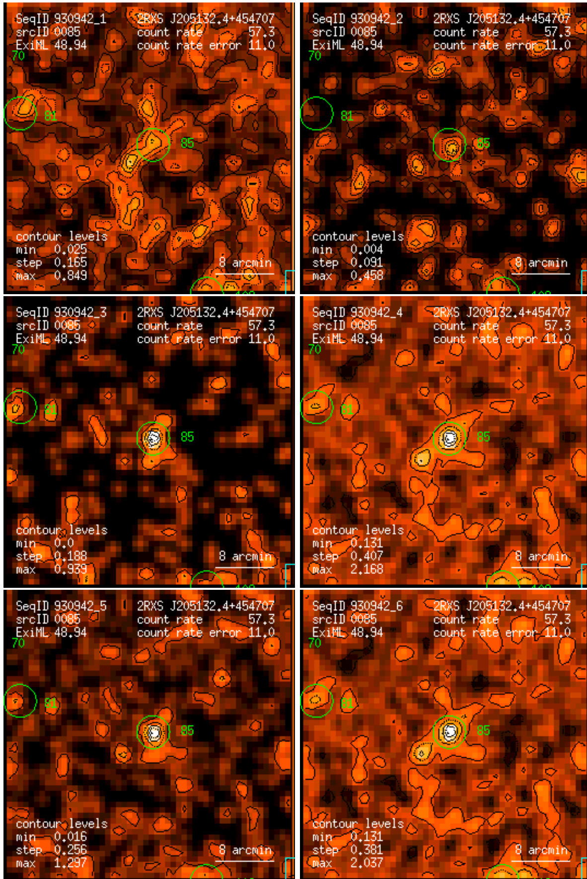
Figure 85: RASS 930942: detection 0085: band rate images, Gaussian filter: (1) PSPC channels 11 – 41, (2) 52 – 90, (3) 91 – 201, (4) 11 – 235, (5) 52 – 201, (6) 11 – 201. Broad band rates in counts/ks. Band rate contour levels in counts/ks/arcmin 2 .
