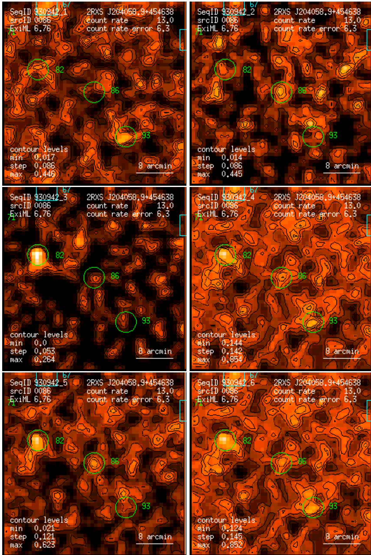
Figure 86: RASS 930942: detection 0086: band rate images, Gaussian filter: (1) PSPC channels 11 – 41, (2) 52 – 90, (3) 91 – 201, (4) 11 – 235, (5) 52 – 201, (6) 11 – 201. Broad band rates in counts/ks. Band rate contour levels in counts/ks/arcmin 2 .
