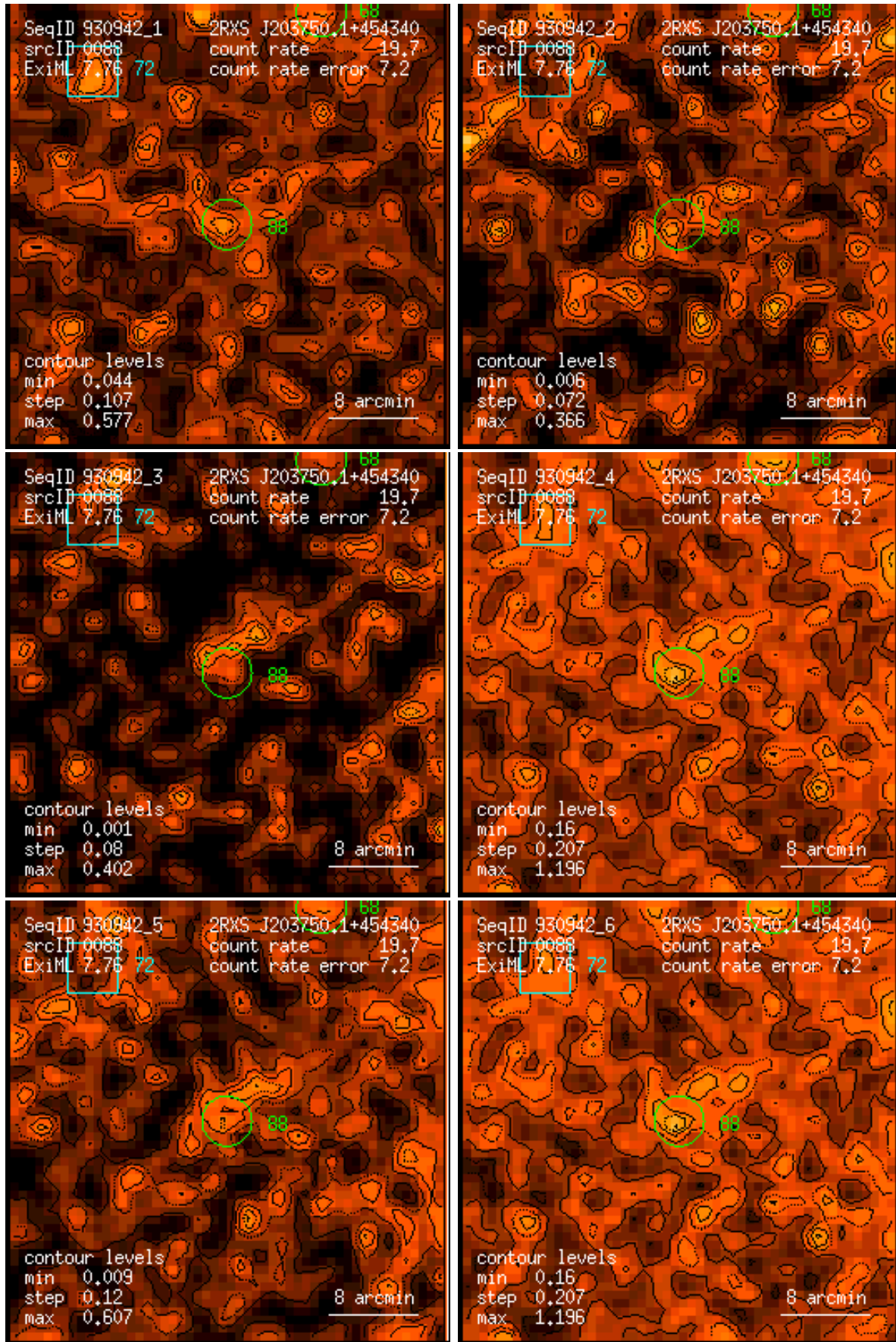
Figure 88: RASS 930942: detection 0088: band rate images, Gaussian filter: (1) PSPC channels 11 – 41, (2) 52 – 90, (3) 91 – 201, (4) 11 – 235, (5) 52 – 201, (6) 11 – 201. Broad band rates in counts/ks. Band rate contour levels in counts/ks/arcmin 2 .
