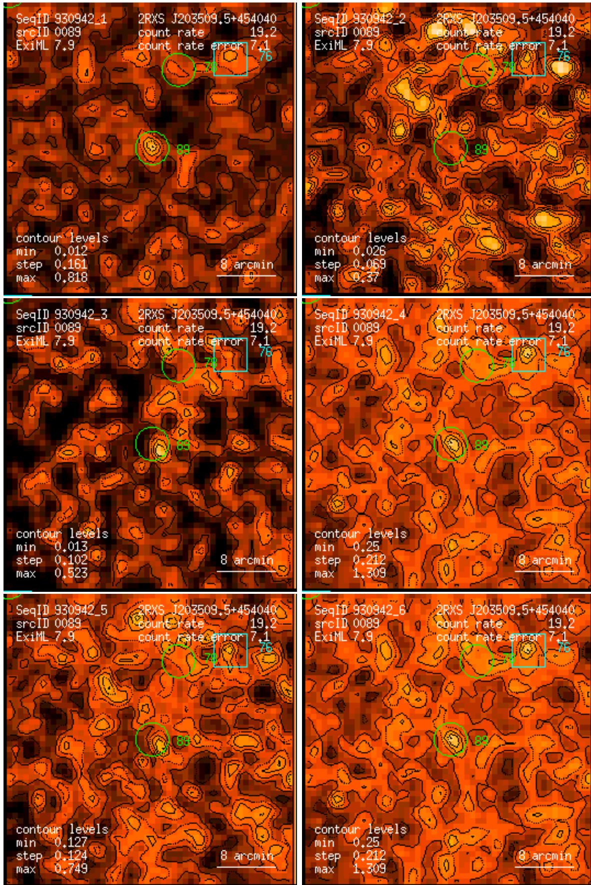
Figure 89: RASS 930942: detection 0089: band rate images, Gaussian filter: (1) PSPC channels 11 – 41, (2) 52 – 90, (3) 91 – 201, (4) 11 – 235, (5) 52 – 201, (6) 11 – 201. Broad band rates in counts/ks. Band rate contour levels in counts/ks/arcmin 2 .
