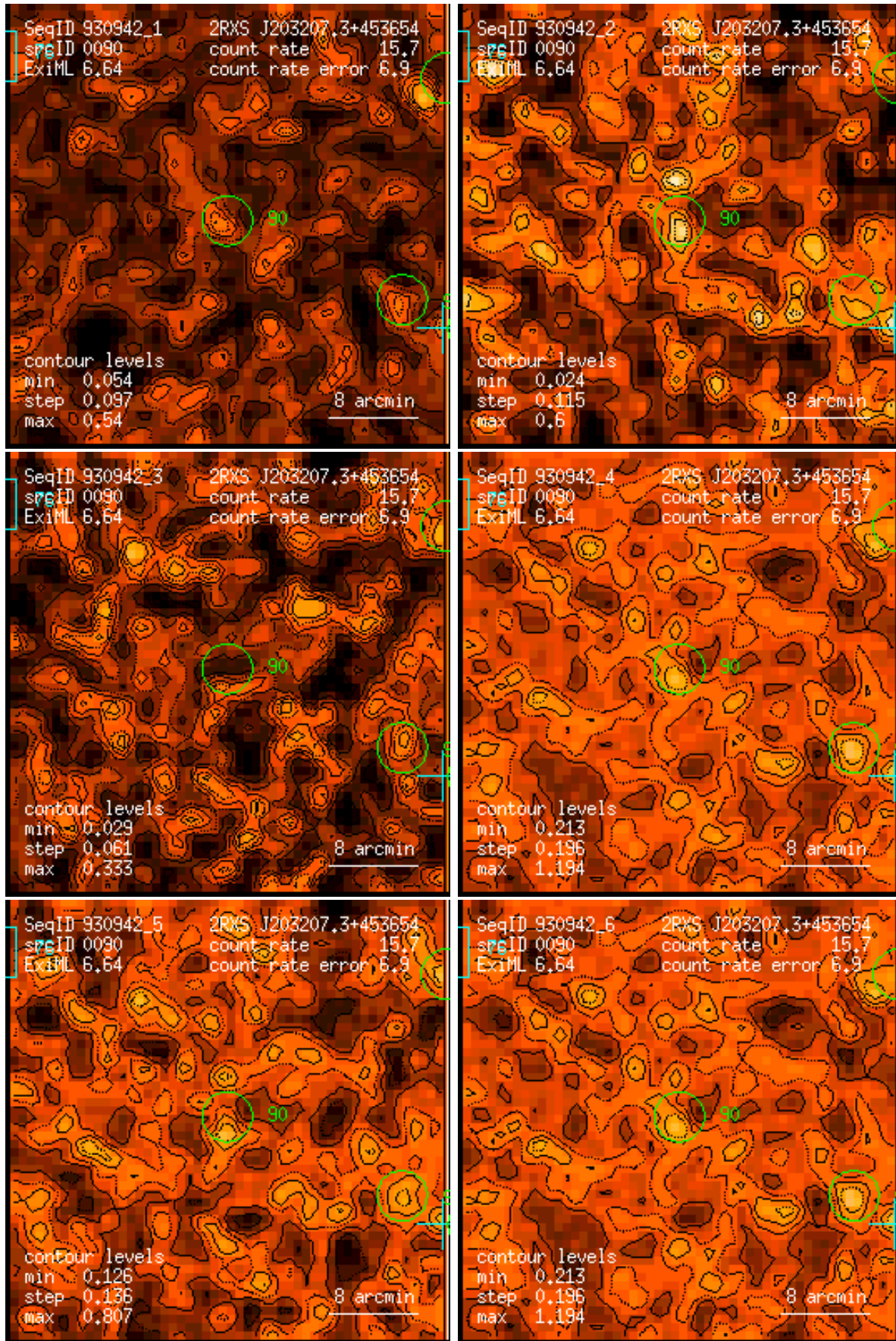
Figure 90: RASS 930942: detection 0090: band rate images, Gaussian filter: (1) PSPC channels 11 – 41, (2) 52 – 90, (3) 91 – 201, (4) 11 – 235, (5) 52 – 201, (6) 11 – 201. Broad band rates in counts/ks. Band rate contour levels in counts/ks/arcmin 2 .
