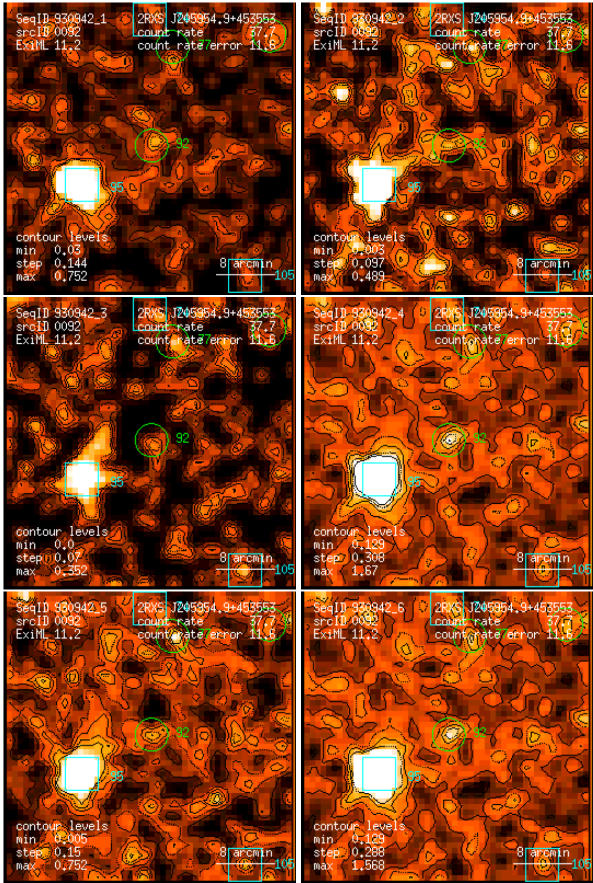
Figure 92: RASS 930942: detection 0092: band rate images, Gaussian filter: (1) PSPC channels 11 – 41, (2) 52 – 90, (3) 91 – 201, (4) 11 – 235, (5) 52 – 201, (6) 11 – 201. Broad band rates in counts/ks. Band rate contour levels in counts/ks/arcmin 2 .
