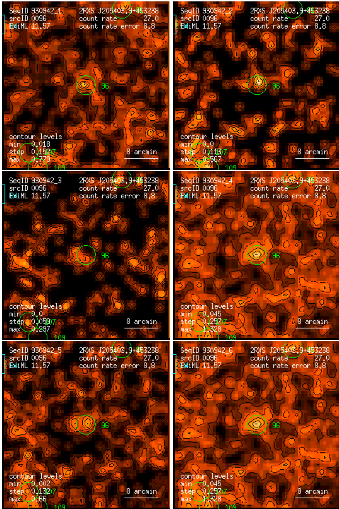
Figure 96: RASS 930942: detection 0096: band rate images, Gaussian filter: (1) PSPC channels 11 – 41, (2) 52 – 90, (3) 91 – 201, (4) 11 – 235, (5) 52 – 201, (6) 11 – 201. Broad band rates in counts/ks. Band rate contour levels in counts/ks/arcmin 2 .
