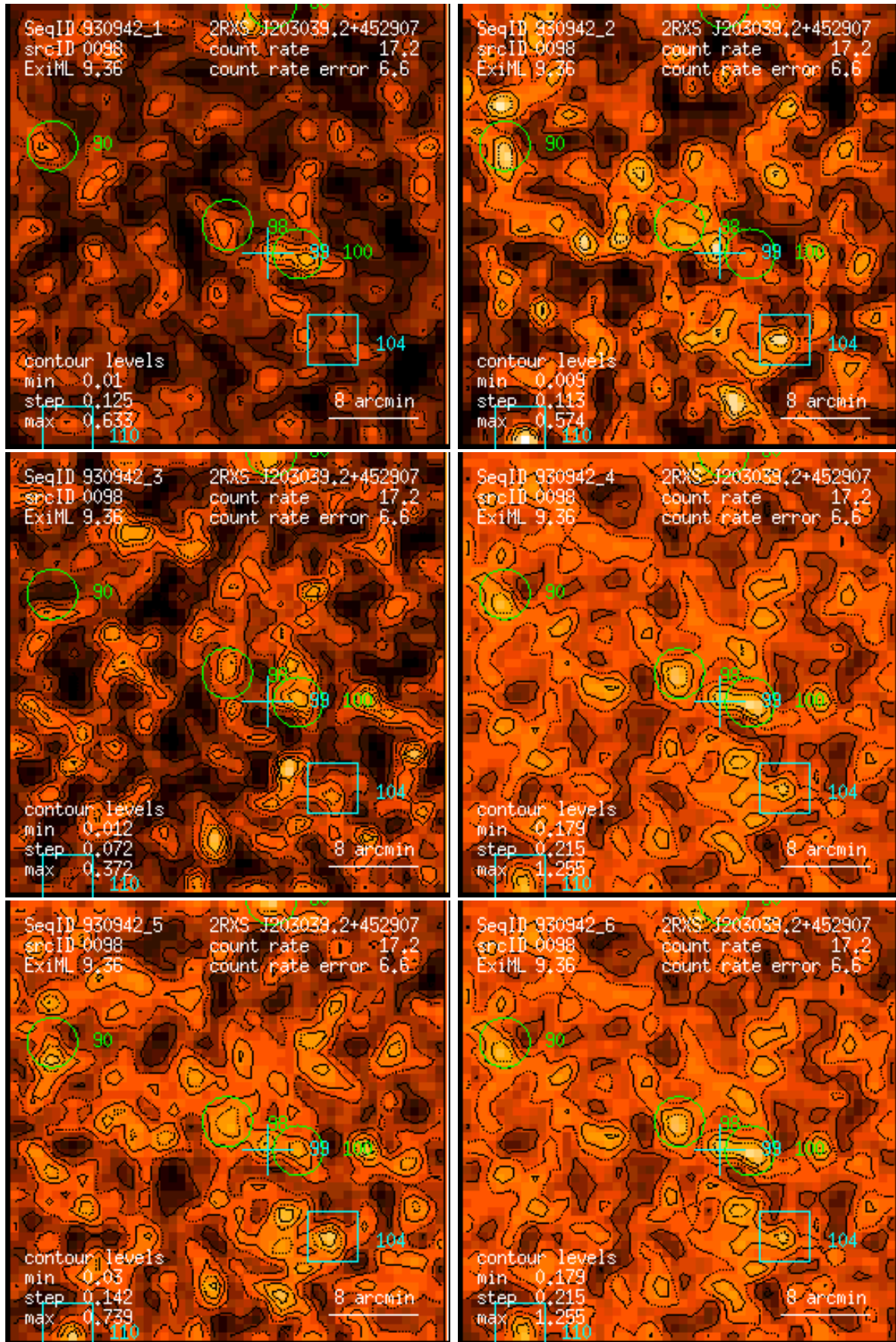
Figure 98: RASS 930942: detection 0098: band rate images, Gaussian filter: (1) PSPC channels 11 – 41, (2) 52 – 90, (3) 91 – 201, (4) 11 – 235, (5) 52 – 201, (6) 11 – 201. Broad band rates in counts/ks. Band rate contour levels in counts/ks/arcmin 2 .
