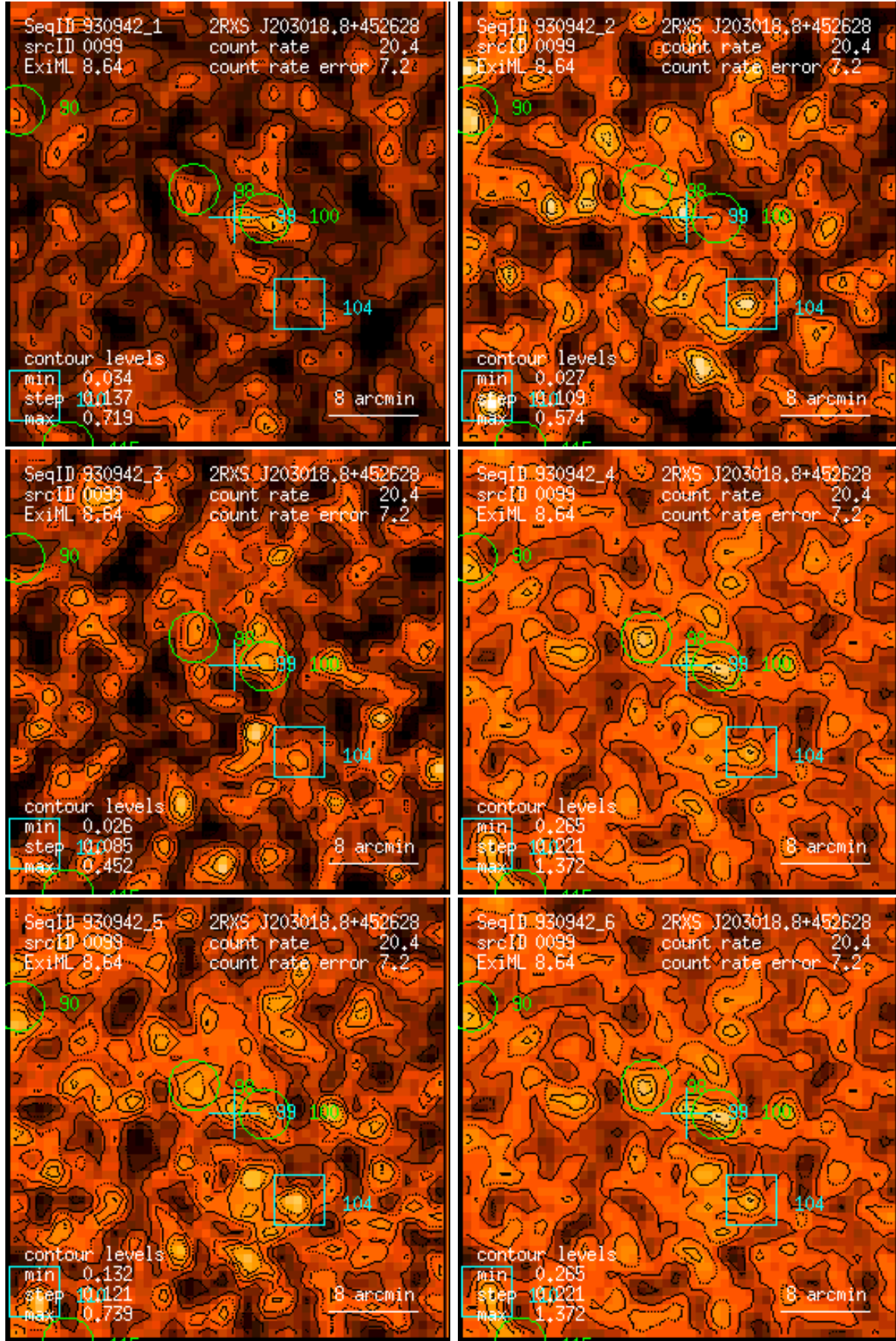
Figure 99: RASS 930942: detection 0099: band rate images, Gaussian filter: (1) PSPC channels 11 – 41, (2) 52 – 90, (3) 91 – 201, (4) 11 – 235, (5) 52 – 201, (6) 11 – 201. Broad band rates in counts/ks. Band rate contour levels in counts/ks/arcmin 2 .
