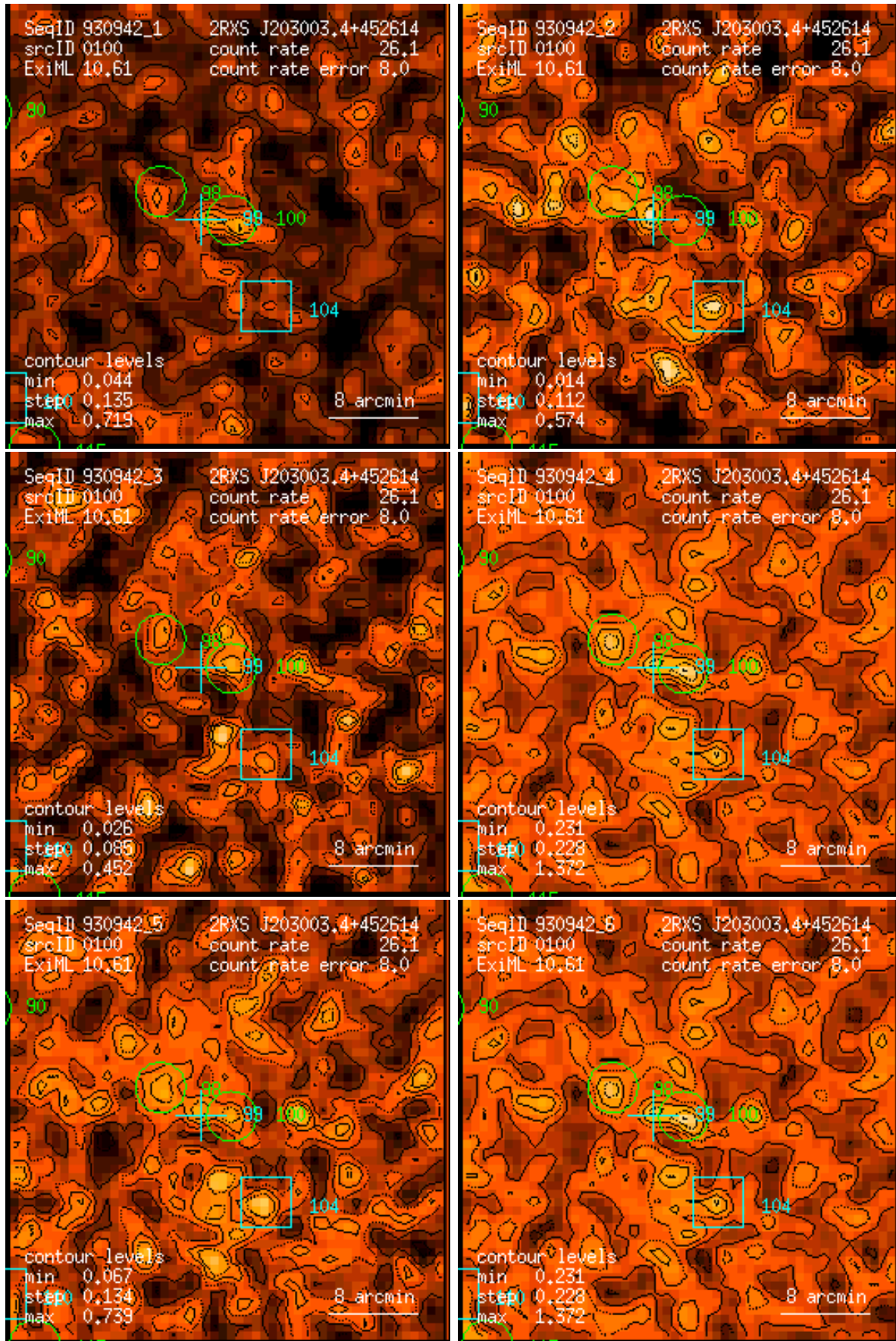
Figure 100: RASS 930942: detection 0100: band rate images, Gaussian filter: (1) PSPC channels 11 – 41, (2) 52 – 90, (3) 91 – 201, (4) 11 – 235, (5) 52 – 201, (6) 11 – 201. Broad band rates in counts/ks. Band rate contour levels in counts/ks/arcmin 2 .
