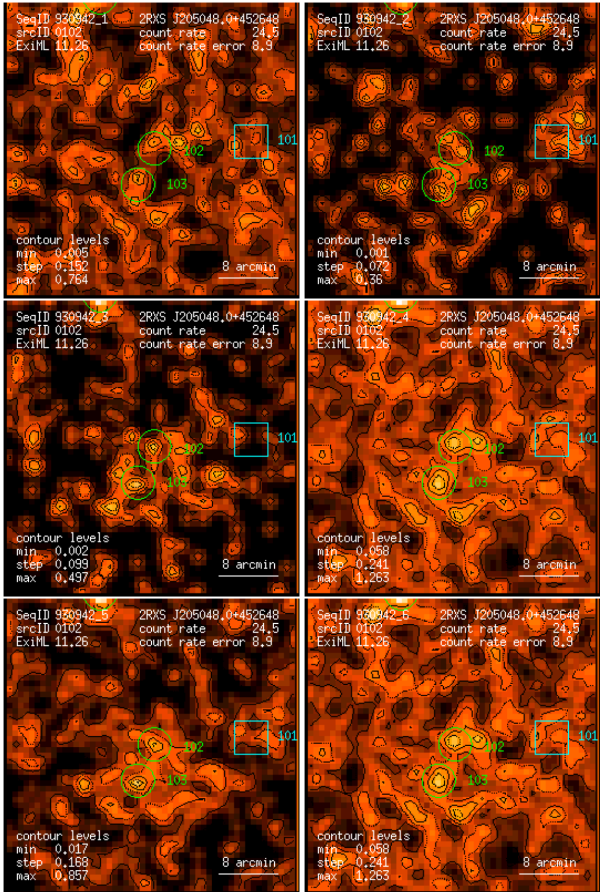
Figure 102: RASS 930942: detection 0102: band rate images, Gaussian filter: (1) PSPC channels 11 – 41, (2) 52 – 90, (3) 91 – 201, (4) 11 – 235, (5) 52 – 201, (6) 11 – 201. Broad band rates in counts/ks. Band rate contour levels in counts/ks/arcmin 2 .
