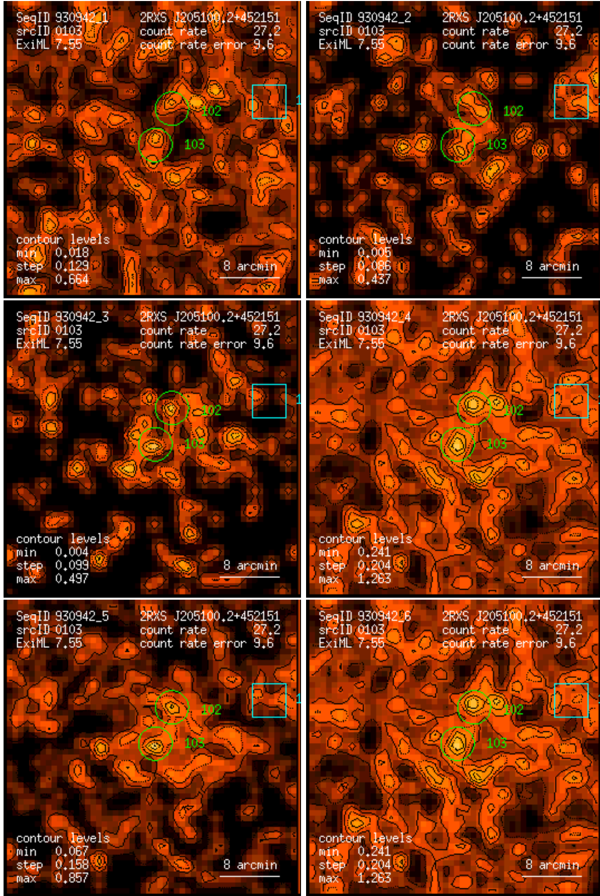
Figure 103: RASS 930942: detection 0103: band rate images, Gaussian filter: (1) PSPC channels 11 – 41, (2) 52 – 90, (3) 91 – 201, (4) 11 – 235, (5) 52 – 201, (6) 11 – 201. Broad band rates in counts/ks. Band rate contour levels in counts/ks/arcmin 2 .
