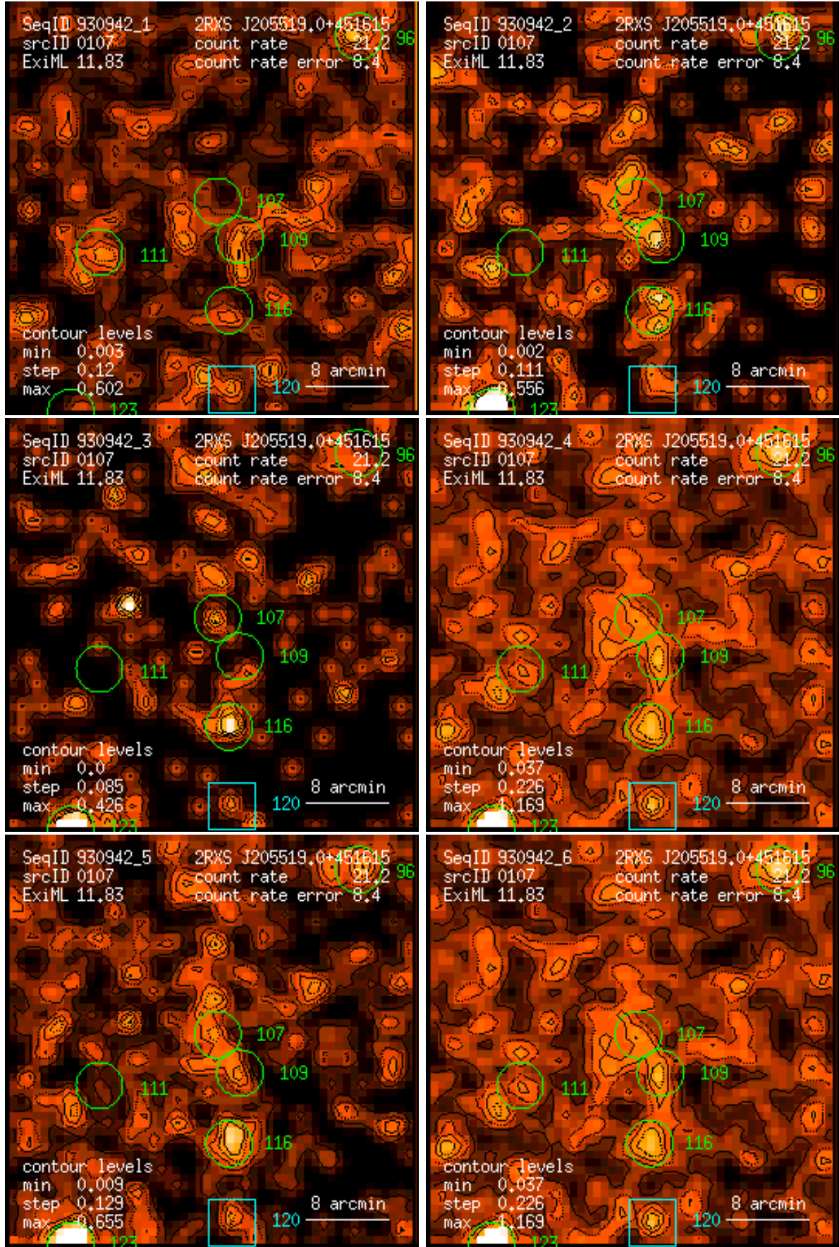
Figure 107: RASS 930942: detection 0107: band rate images, Gaussian filter: (1) PSPC channels 11 – 41, (2) 52 – 90, (3) 91 – 201, (4) 11 – 235, (5) 52 – 201, (6) 11 – 201. Broad band rates in counts/ks. Band rate contour levels in counts/ks/arcmin 2 .
