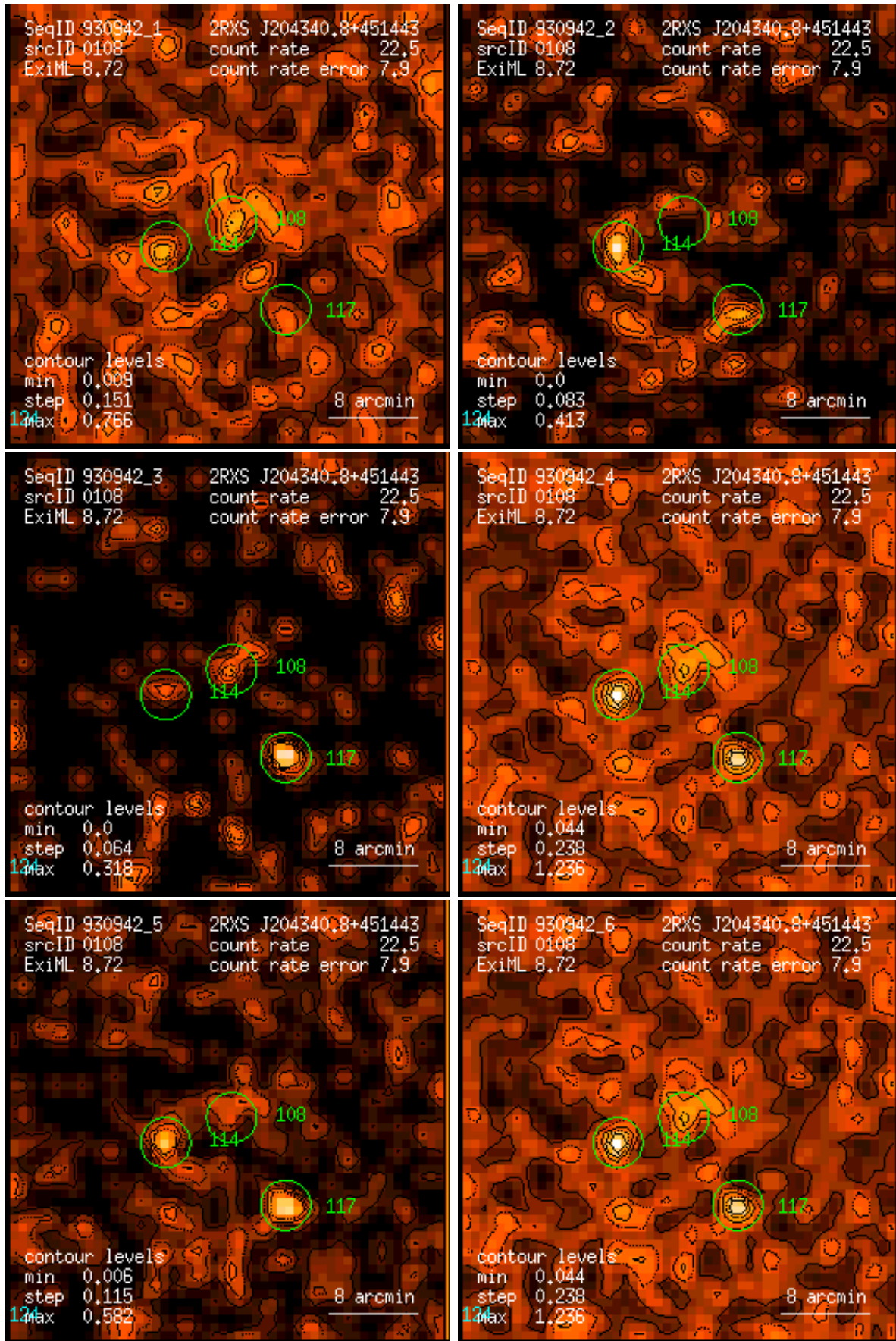
Figure 108: RASS 930942: detection 0108: band rate images, Gaussian filter: (1) PSPC channels 11 – 41, (2) 52 – 90, (3) 91 – 201, (4) 11 – 235, (5) 52 – 201, (6) 11 – 201. Broad band rates in counts/ks. Band rate contour levels in counts/ks/arcmin 2 .
