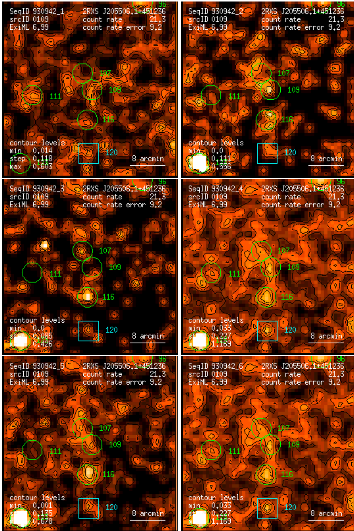
Figure 109: RASS 930942: detection 0109: band rate images, Gaussian filter: (1) PSPC channels 11 – 41, (2) 52 – 90, (3) 91 – 201, (4) 11 – 235, (5) 52 – 201, (6) 11 – 201. Broad band rates in counts/ks. Band rate contour levels in counts/ks/arcmin 2 .
