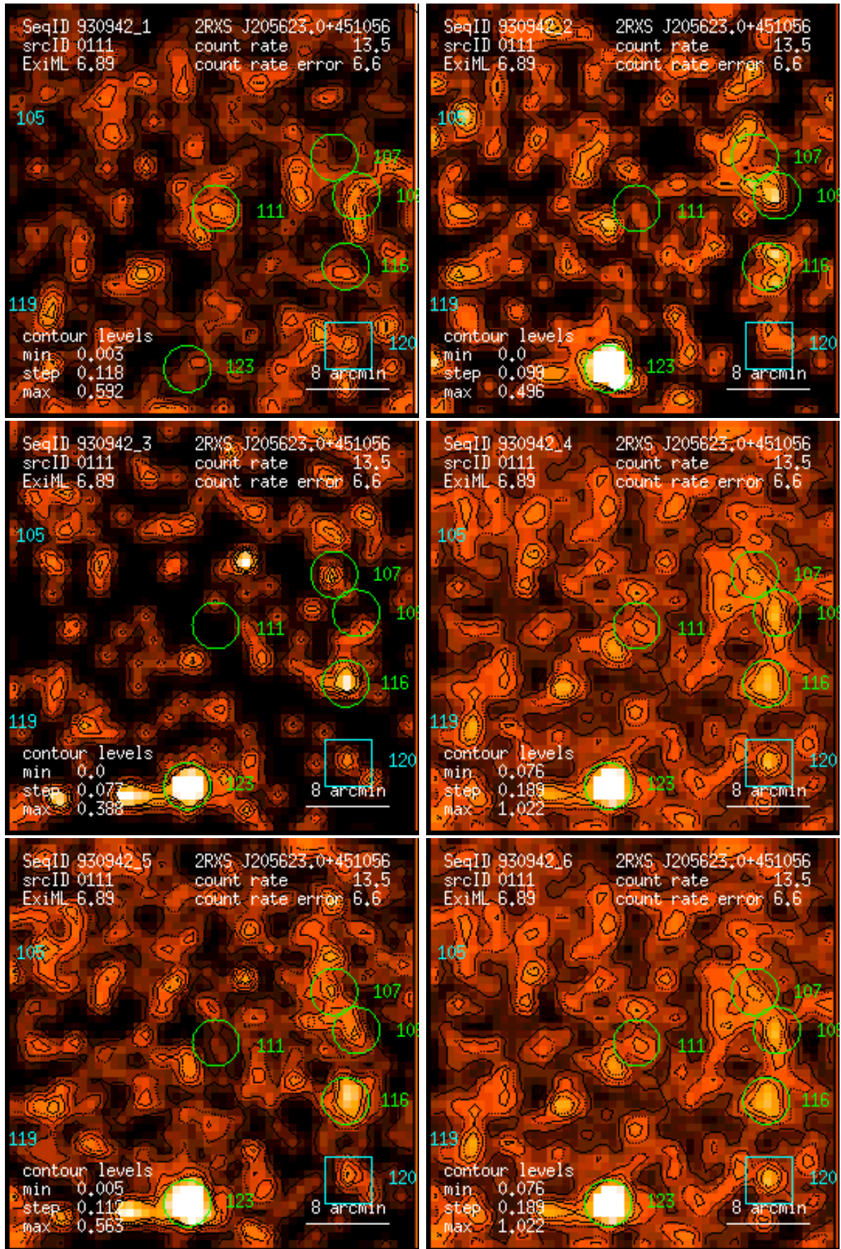
Figure 111: RASS 930942: detection 0111: band rate images, Gaussian filter: (1) PSPC channels 11 – 41, (2) 52 – 90, (3) 91 – 201, (4) 11 – 235, (5) 52 – 201, (6) 11 – 201. Broad band rates in counts/ks. Band rate contour levels in counts/ks/arcmin 2 .
