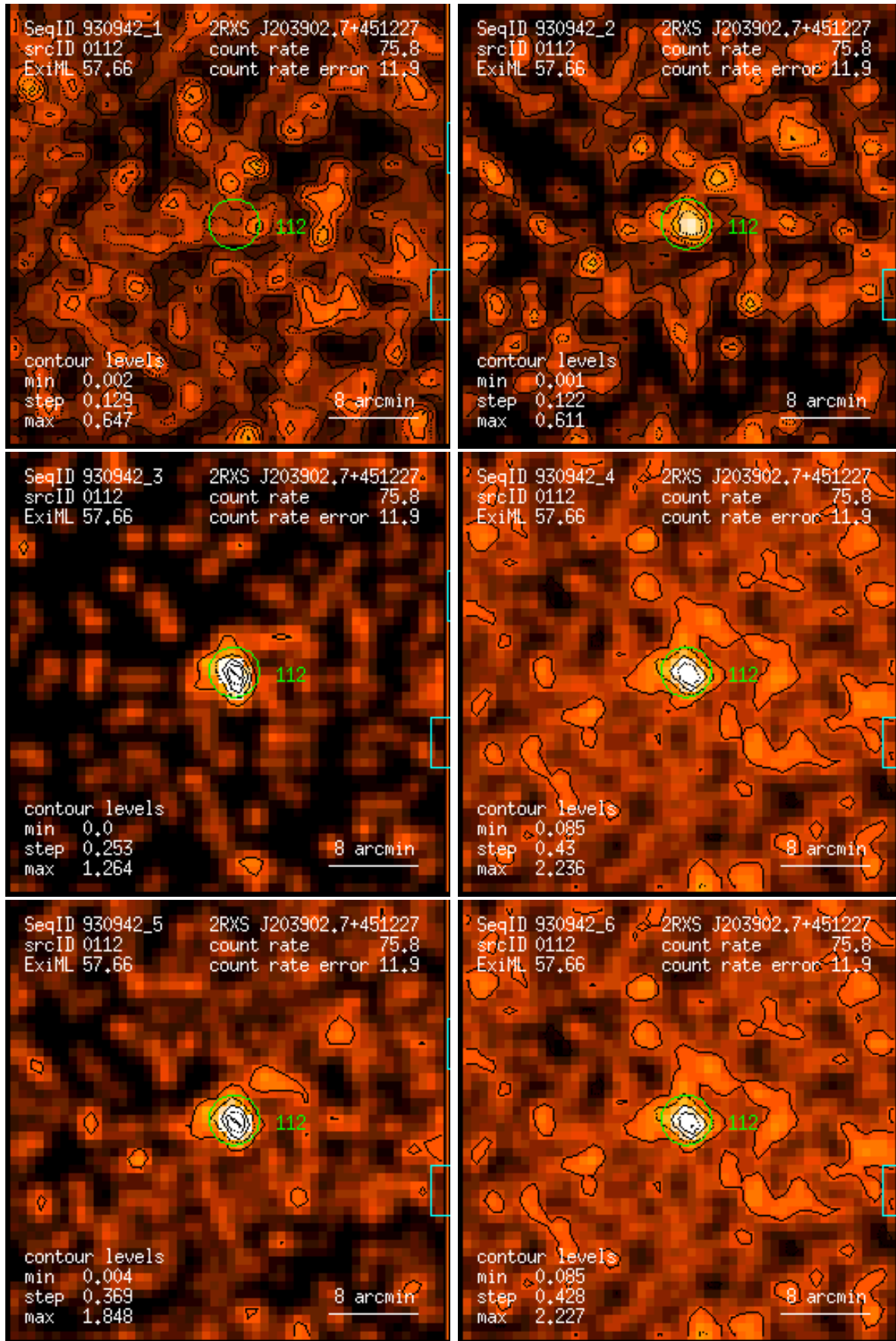
Figure 112: RASS 930942: detection 0112: band rate images, Gaussian filter: (1) PSPC channels 11 – 41, (2) 52 – 90, (3) 91 – 201, (4) 11 – 235, (5) 52 – 201, (6) 11 – 201. Broad band rates in counts/ks. Band rate contour levels in counts/ks/arcmin 2 .
