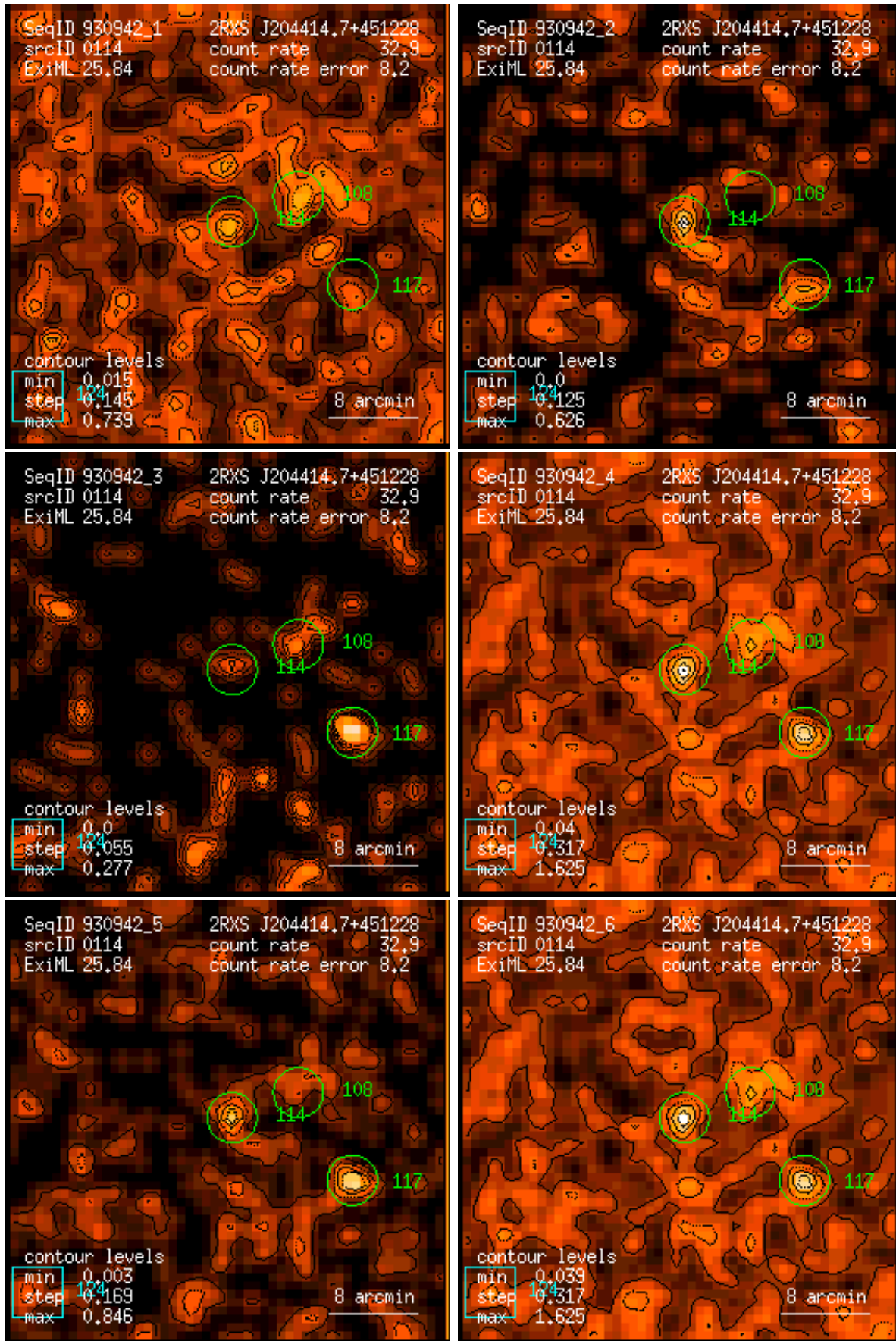
Figure 114: RASS 930942: detection 0114: band rate images, Gaussian filter: (1) PSPC channels 11 – 41, (2) 52 – 90, (3) 91 – 201, (4) 11 – 235, (5) 52 – 201, (6) 11 – 201. Broad band rates in counts/ks. Band rate contour levels in counts/ks/arcmin 2 .
