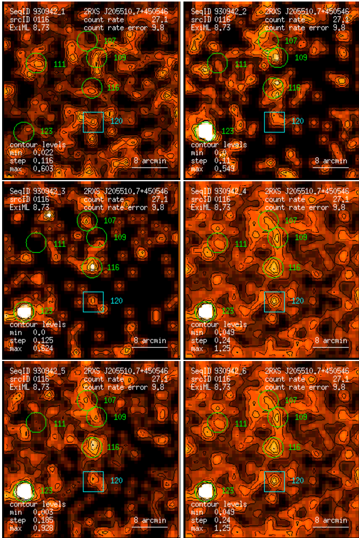
Figure 116: RASS 930942: detection 0116: band rate images, Gaussian filter: (1) PSPC channels 11 – 41, (2) 52 – 90, (3) 91 – 201, (4) 11 – 235, (5) 52 – 201, (6) 11 – 201. Broad band rates in counts/ks. Band rate contour levels in counts/ks/arcmin 2 .
