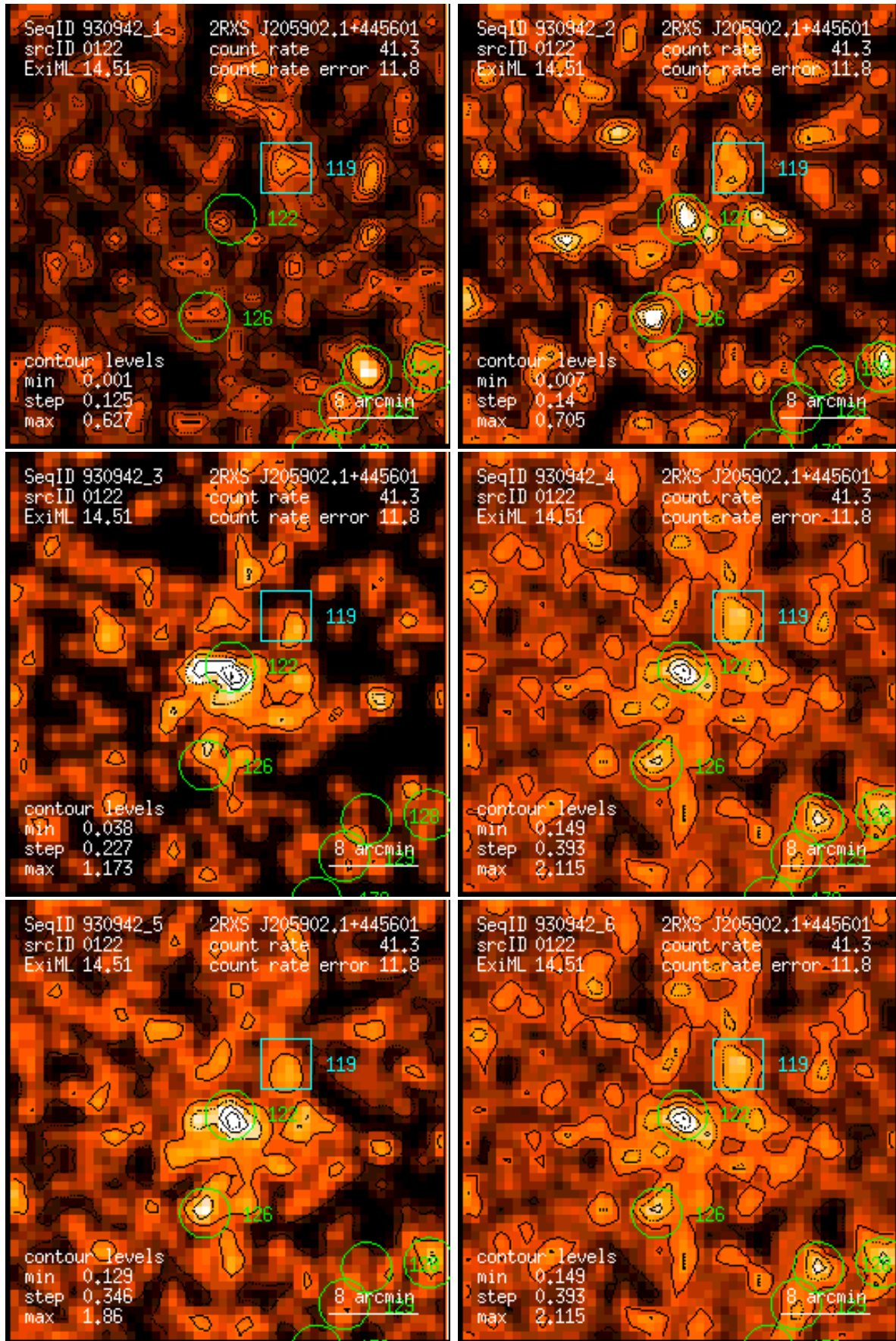
Figure 122: RASS 930942: detection 0122: band rate images, Gaussian filter: (1) PSPC channels 11 – 41, (2) 52 – 90, (3) 91 – 201, (4) 11 – 235, (5) 52 – 201, (6) 11 – 201. Broad band rates in counts/ks. Band rate contour levels in counts/ks/arcmin 2 .
