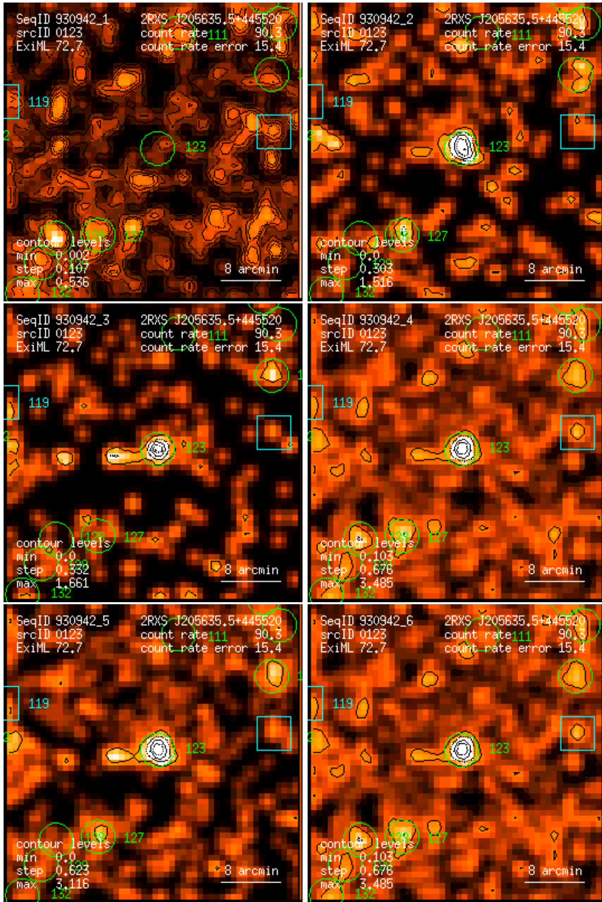
Figure 123: RASS 930942: detection 0123: band rate images, Gaussian filter: (1) PSPC channels 11 – 41, (2) 52 – 90, (3) 91 – 201, (4) 11 – 235, (5) 52 – 201, (6) 11 – 201. Broad band rates in counts/ks. Band rate contour levels in counts/ks/arcmin 2 .
