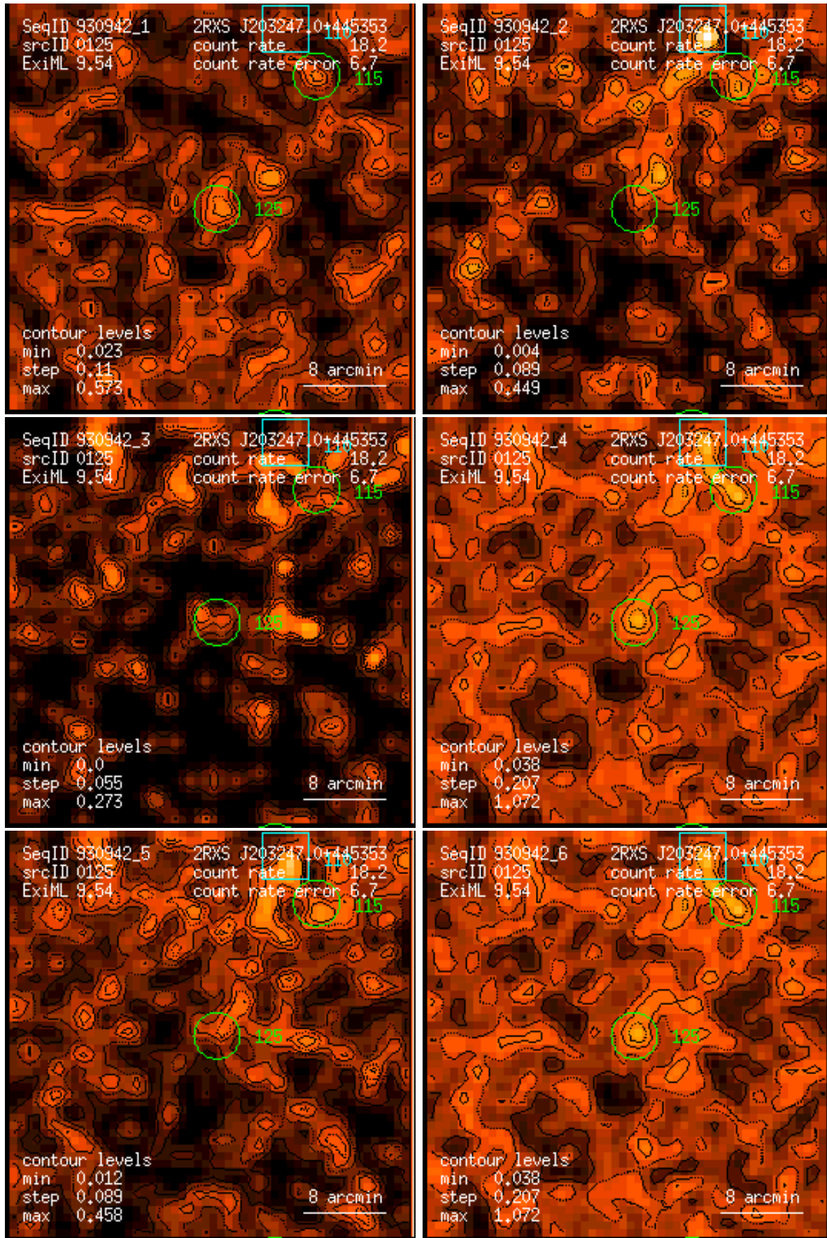
Figure 125: RASS 930942: detection 0125: band rate images, Gaussian filter: (1) PSPC channels 11 – 41, (2) 52 – 90, (3) 91 – 201, (4) 11 – 235, (5) 52 – 201, (6) 11 – 201. Broad band rates in counts/ks. Band rate contour levels in counts/ks/arcmin 2 .
