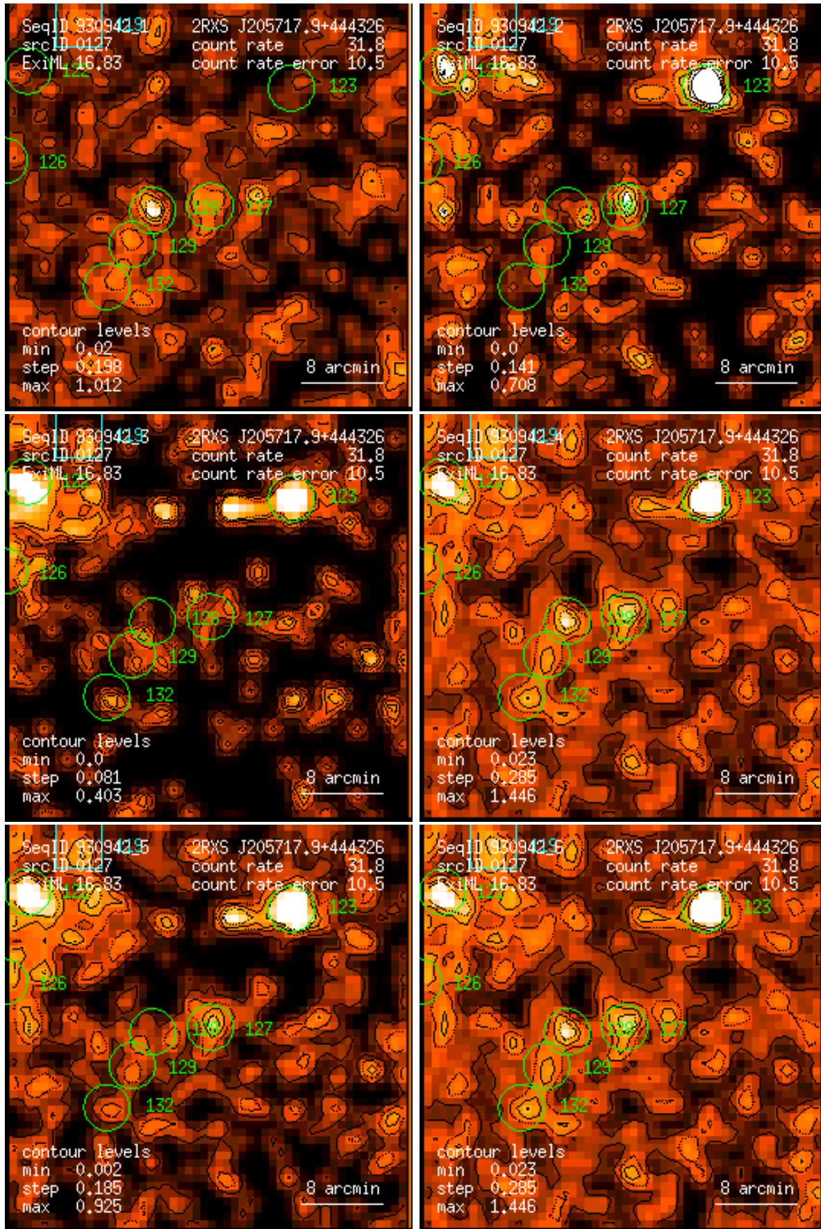
Figure 127: RASS 930942: detection 0127: band rate images, Gaussian filter: (1) PSPC channels 11 – 41, (2) 52 – 90, (3) 91 – 201, (4) 11 – 235, (5) 52 – 201, (6) 11 – 201. Broad band rates in counts/ks. Band rate contour levels in counts/ks/arcmin 2 .
