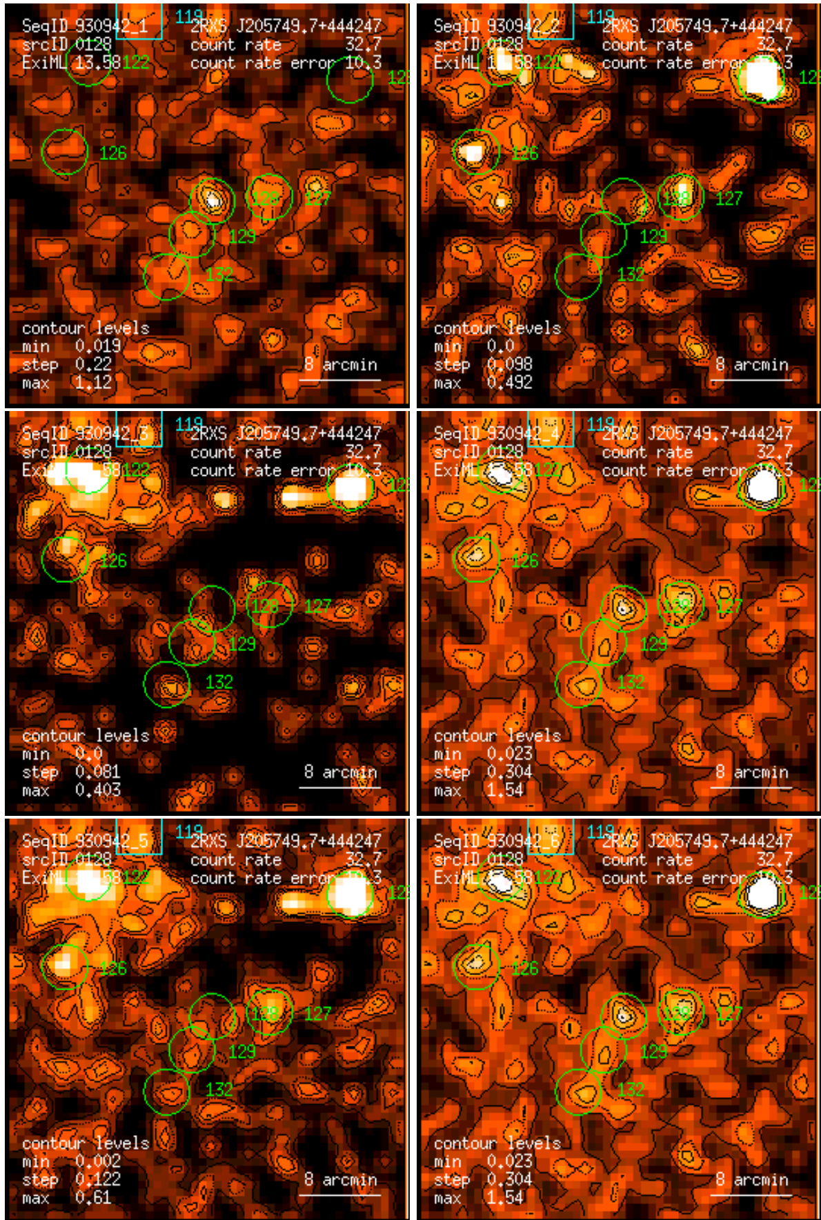
Figure 128: RASS 930942: detection 0128: band rate images, Gaussian filter: (1) PSPC channels 11 – 41, (2) 52 – 90, (3) 91 – 201, (4) 11 – 235, (5) 52 – 201, (6) 11 – 201. Broad band rates in counts/ks. Band rate contour levels in counts/ks/arcmin 2 .
