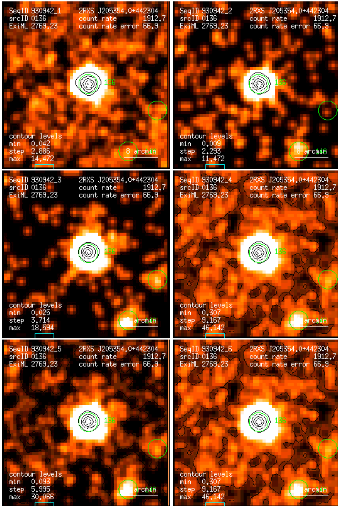
Figure 136: RASS 930942: detection 0136: band rate images, Gaussian filter: (1) PSPC channels 11 – 41, (2) 52 – 90, (3) 91 – 201, (4) 11 – 235, (5) 52 – 201, (6) 11 – 201. Broad band rates in counts/ks. Band rate contour levels in counts/ks/arcmin 2 .
