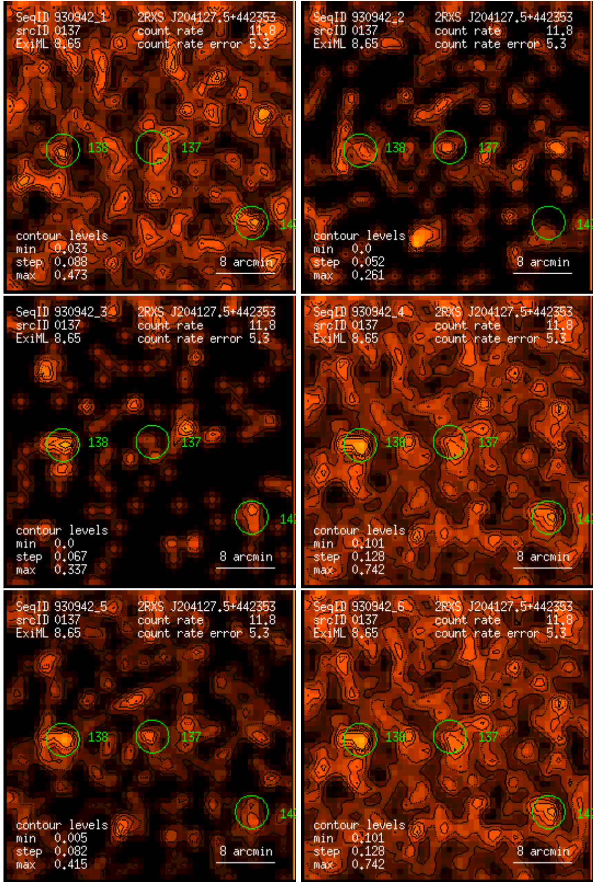
Figure 137: RASS 930942: detection 0137: band rate images, Gaussian filter: (1) PSPPC channels 11 – 41, (2) 52 – 90, (3) 91 – 201, (4) 11 – 235, (5) 52 – 201, (6) 11 – 201. Broad band rates in counts/ks. Band rate contour levels in counts/ks/arcmin 2 .
