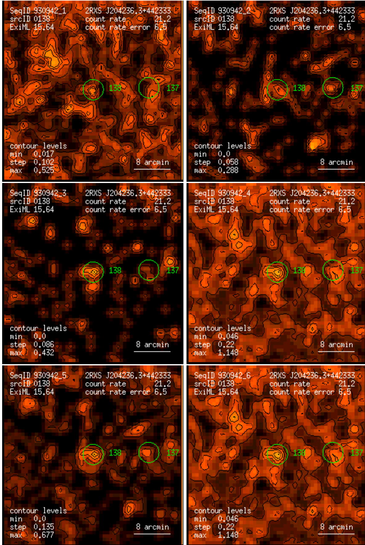
Figure 138: RASS 930942: detection 0138: band rate images, Gaussian filter: (1) PSPC channels 11 – 41, (2) 52 – 90, (3) 91 – 201, (4) 11 – 235, (5) 52 – 201, (6) 11 – 201. Broad band rates in counts/ks. Band rate contour levels in counts/ks/arcmin 2 .
