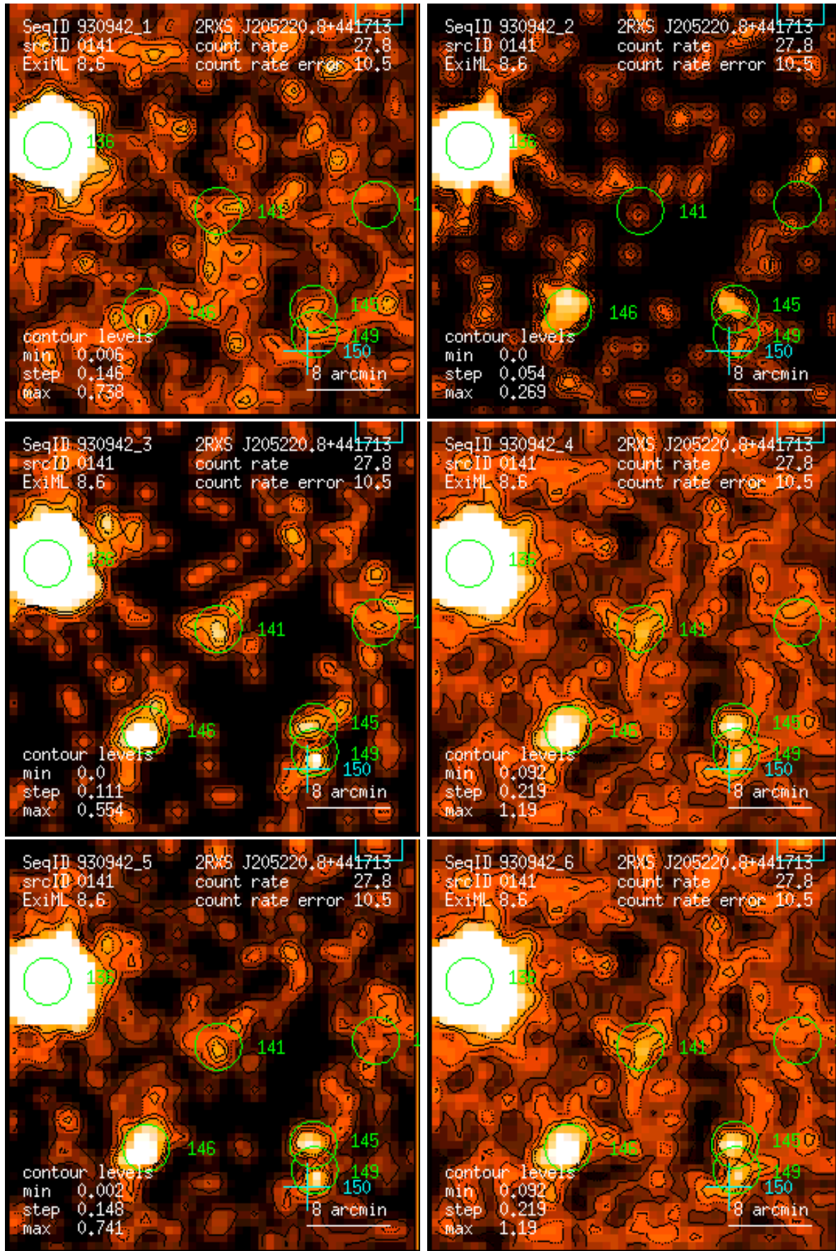
Figure 141: RASS 930942: detection 0141: band rate images, Gaussian filter: (1) PSPC channels 11 – 41, (2) 52 – 90, (3) 91 – 201, (4) 11 – 235, (5) 52 – 201, (6) 11 – 201. Broad band rates in counts/ks. Band rate contour levels in counts/ks/arcmin 2 .
