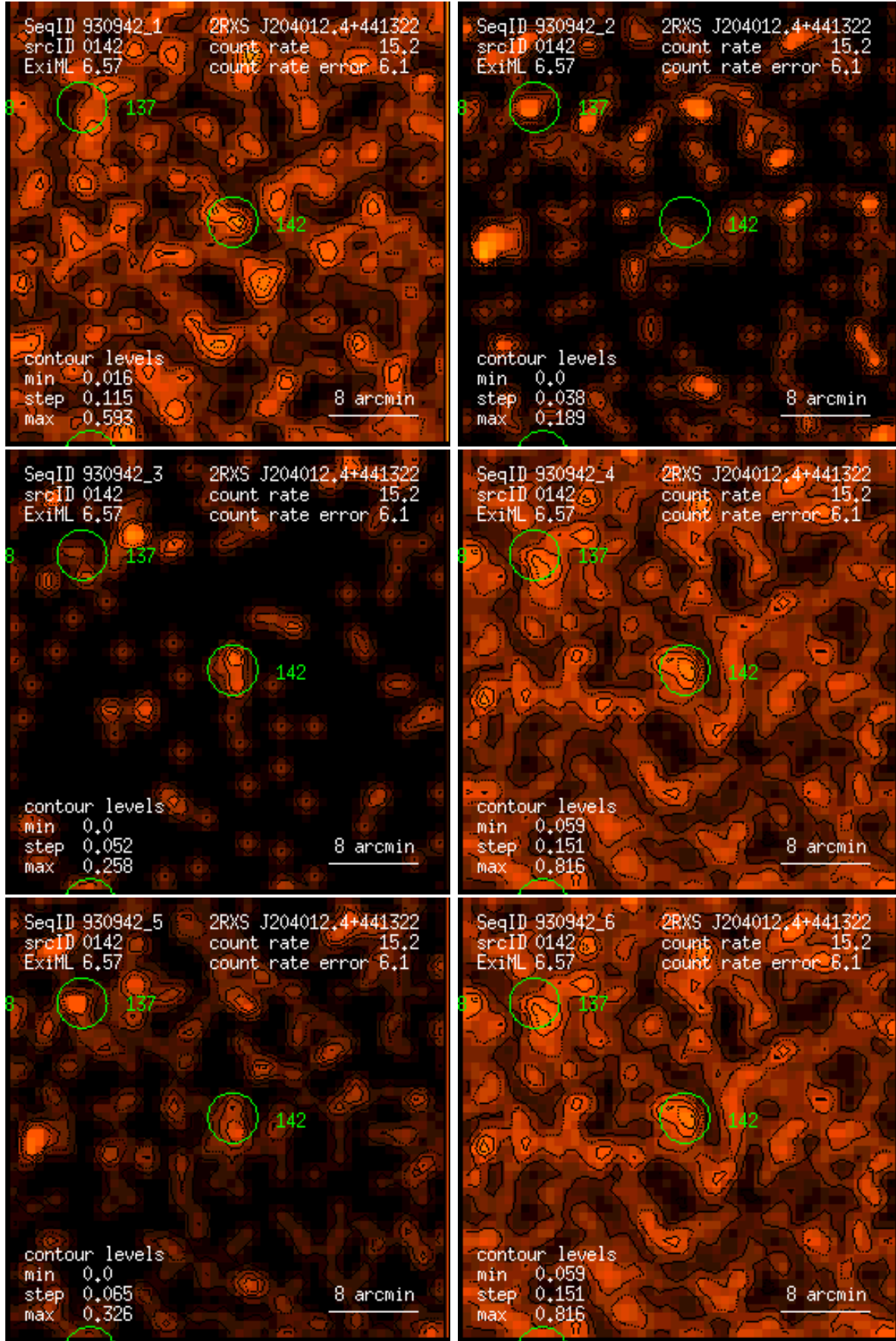
Figure 142: RASS 930942: detection 0142: band rate images, Gaussian filter: (1) PSPC channels 11 – 41, (2) 52 – 90, (3) 91 – 201, (4) 11 – 235, (5) 52 – 201, (6) 11 – 201. Broad band rates in counts/ks. Band rate contour levels in counts/ks/arcmin 2 .
