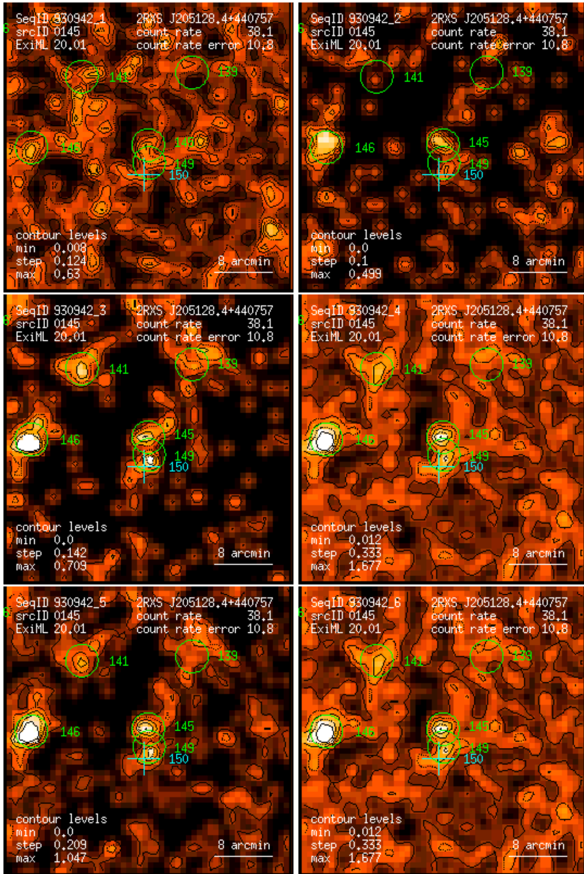
Figure 145: RASS 930942: detection 0145: band rate images, Gaussian filter: (1) PSPC channels 11 – 41, (2) 52 – 90, (3) 91 – 201, (4) 11 – 235, (5) 52 – 201, (6) 11 – 201. Broad band rates in counts/ks. Band rate contour levels in counts/ks/arcmin 2 .
