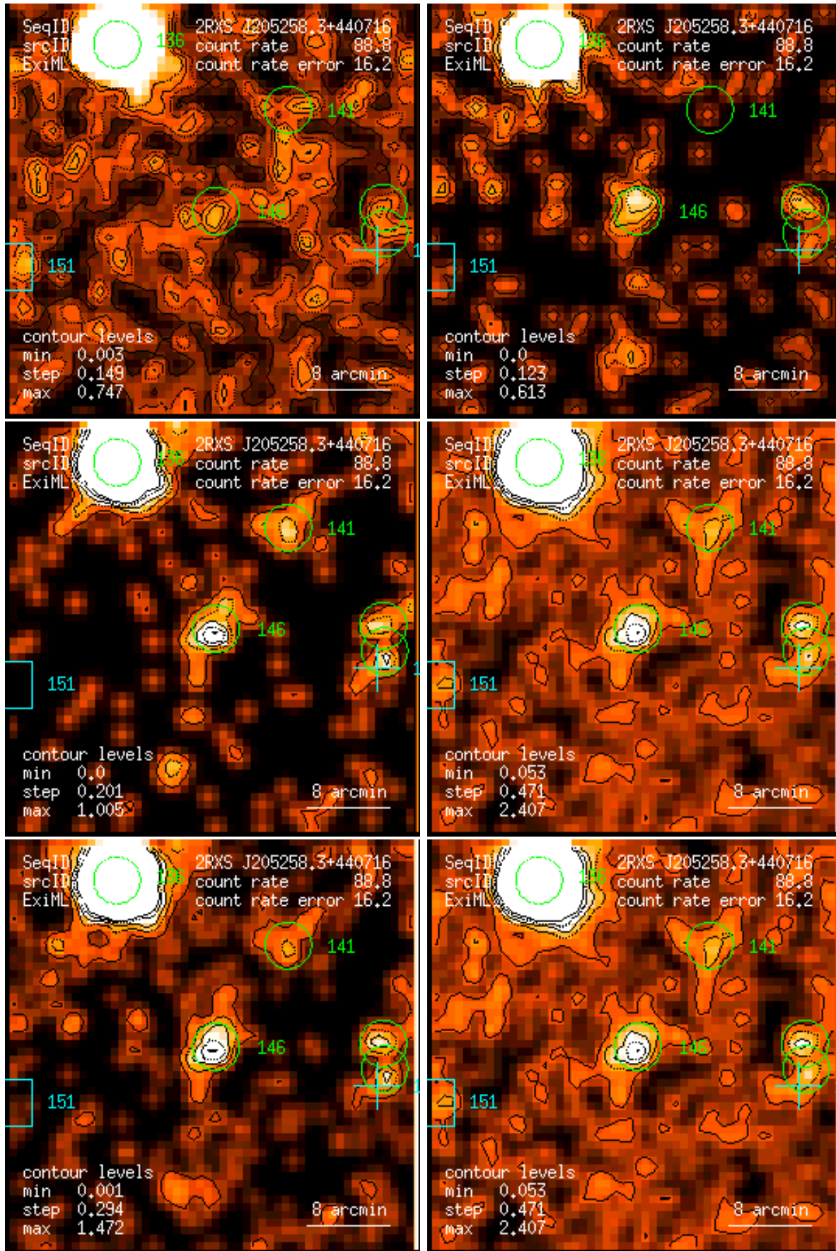
Figure 146: RASS 930942: detection 0146: band rate images, Gaussian filter: (1) PSPC channels 11 – 41, (2) 52 – 90, (3) 91 – 201, (4) 11 – 235, (5) 52 – 201, (6) 11 – 201. Broad band rates in counts/ks. Band rate contour levels in counts/ks/arcmin 2 .
