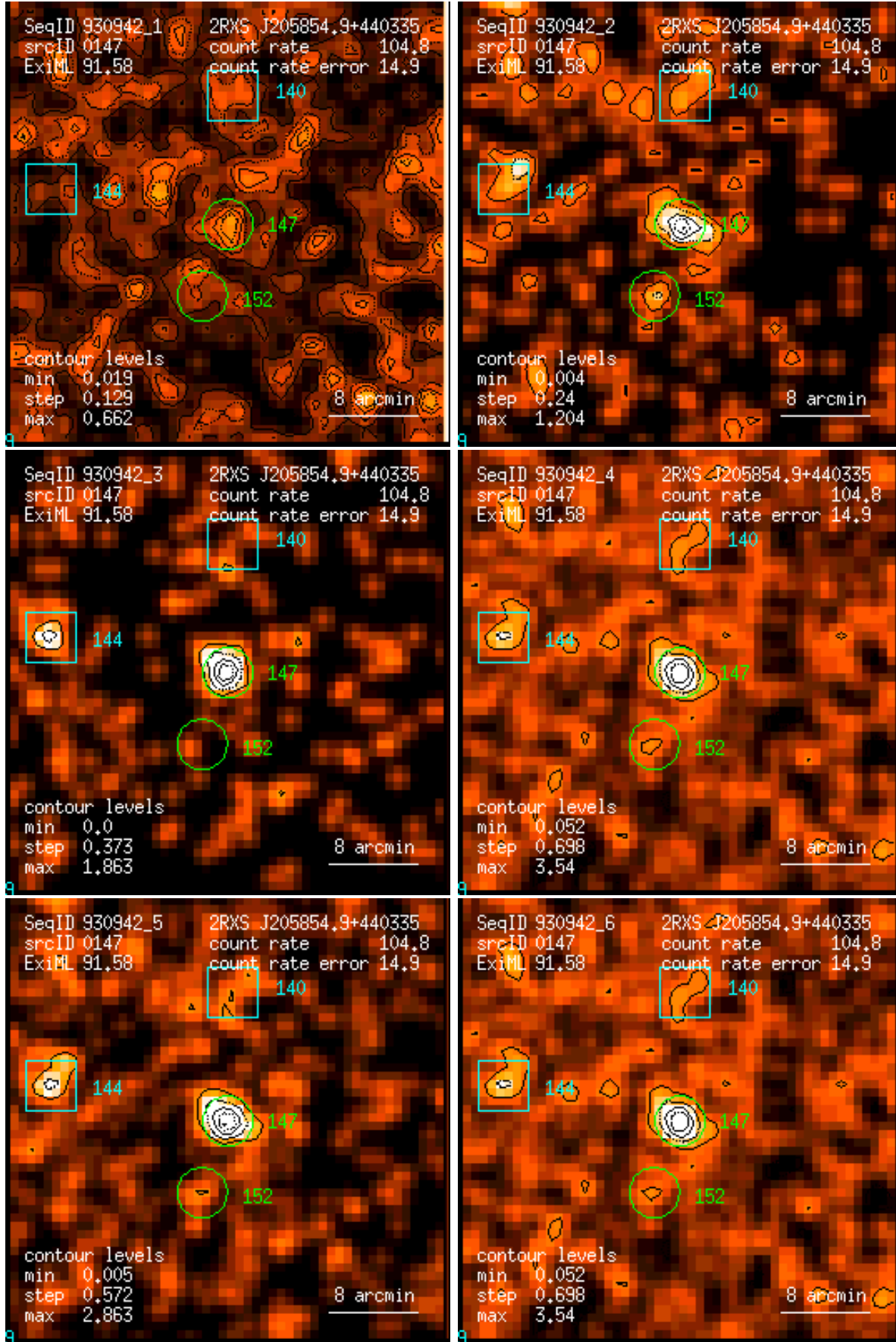
Figure 147: RASS 930942: detection 0147: band rate images, Gaussian filter: (1) PSPC channels 11 – 41, (2) 52 – 90, (3) 91 – 201, (4) 11 – 235, (5) 52 – 201, (6) 11 – 201. Broad band rates in counts/ks. Band rate contour levels in counts/ks/arcmin 2 .
