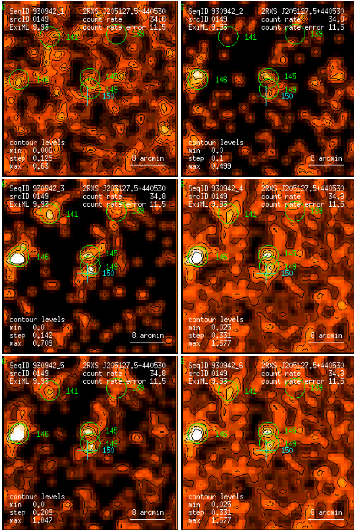
Figure 149: RASS 930942: detection 0149: band rate images, Gaussian filter: (1) PSPC channels 11 – 41, (2) 52 – 90, (3) 91 – 201, (4) 11 – 235, (5) 52 – 201, (6) 11 – 201. Broad band rates in counts/ks. Band rate contour levels in counts/ks/arcmin 2 .
