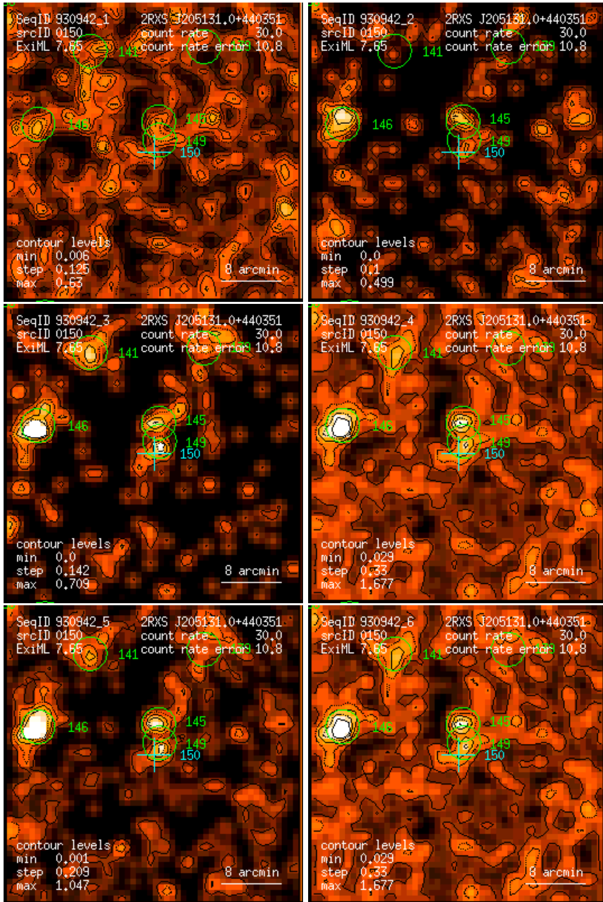
Figure 150: RASS 930942: detection 0150: band rate images, Gaussian filter: (1) PSPC channels 11 – 41, (2) 52 – 90, (3) 91 – 201, (4) 11 – 235, (5) 52 – 201, (6) 11 – 201. Broad band rates in counts/ks. Band rate contour levels in counts/ks/arcmin 2 .
