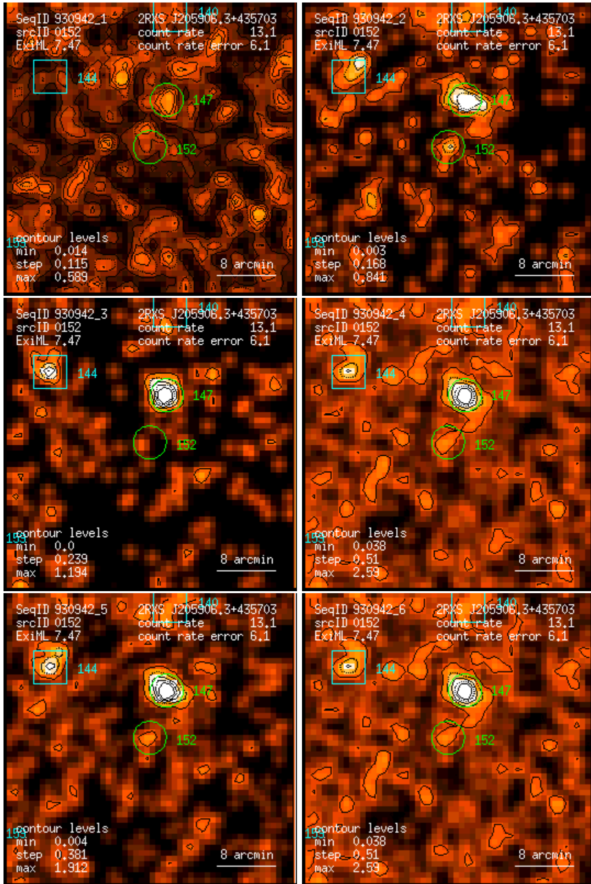
Figure 152: RASS 930942: detection 0152: band rate images, Gaussian filter: (1) PSPC channels 11 – 41, (2) 52 – 90, (3) 91 – 201, (4) 11 – 235, (5) 52 – 201, (6) 11 – 201. Broad band rates in counts/ks. Band rate contour levels in counts/ks/arcmin 2 .
