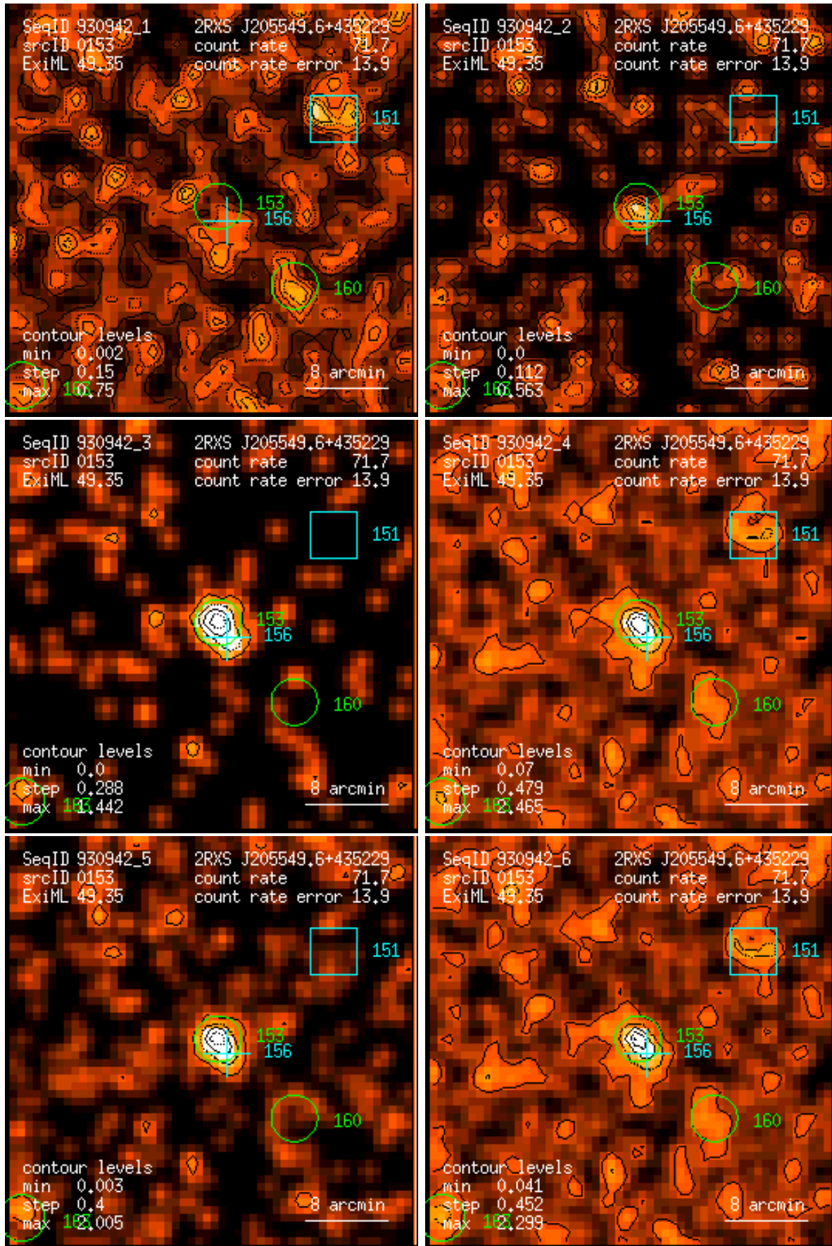
Figure 153: RASS 930942: detection 0153: band rate images, Gaussian filter: (1) PSPC channels 11 – 41, (2) 52 – 90, (3) 91 – 201, (4) 11 – 235, (5) 52 – 201, (6) 11 – 201. Broad band rates in counts/ks. Band rate contour levels in counts/ks/arcmin 2 .
