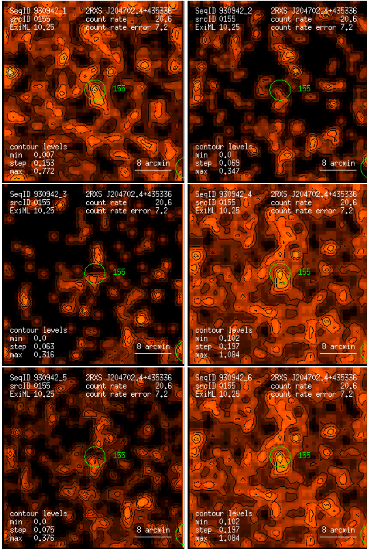
Figure 155: RASS 930942: detection 0155: band rate images, Gaussian filter: (1) PSPC channels 11 – 41, (2) 52 – 90, (3) 91 – 201, (4) 11 – 235, (5) 52 – 201, (6) 11 – 201. Broad band rates in counts/ks. Band rate contour levels in counts/ks/arcmin 2 .
