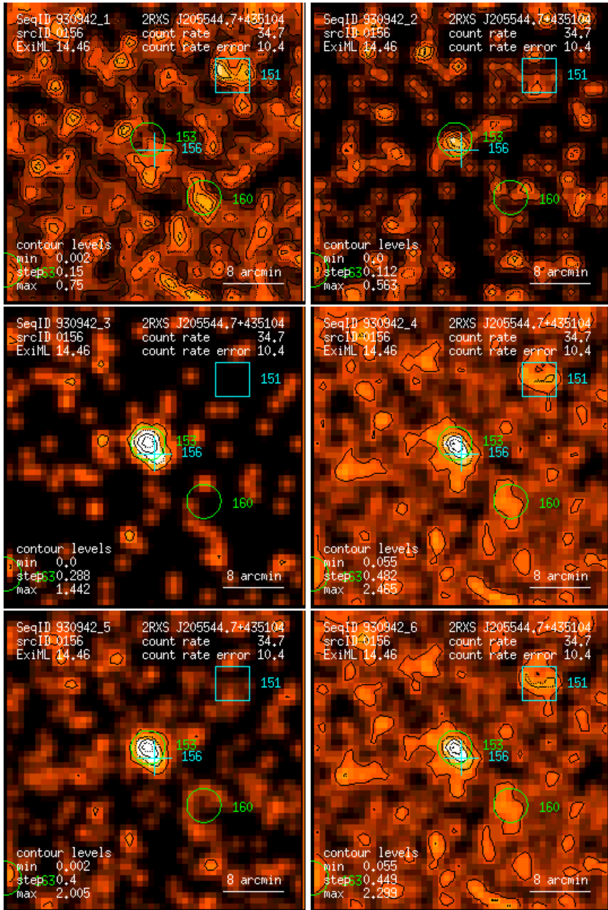
Figure 156: RASS 930942: detection 0156: band rate images, Gaussian filter: (1) PSPC channels 11 – 41, (2) 52 – 90, (3) 91 – 201, (4) 11 – 235, (5) 52 – 201, (6) 11 – 201. Broad band rates in counts/ks. Band rate contour levels in counts/ks/arcmin 2 .
