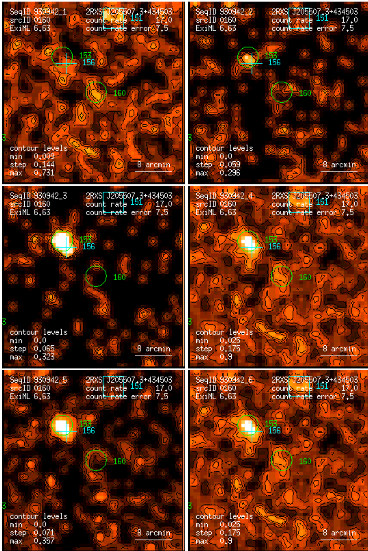
Figure 160: RASS 930942: detection 0160: band rate images, Gaussian filter: (1) PSPC channels 11 – 41, (2) 52 – 90, (3) 91 – 201, (4) 11 – 235, (5) 52 – 201, (6) 11 – 201. Broad band rates in counts/ks. Band rate contour levels in counts/ks/arcmin 2 .
