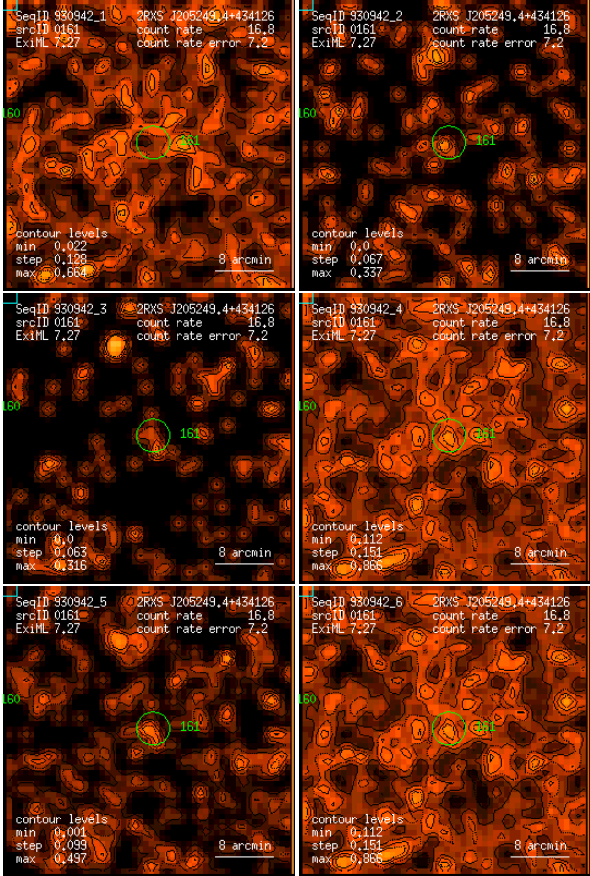
Figure 161: RASS 930942: detection 0161: band rate images, Gaussian filter: (1) PSPC channels 11 – 41, (2) 52 – 90, (3) 91 – 201, (4) 11 – 235, (5) 52 – 201, (6) 11 – 201. Broad band rates in counts/ks. Band rate contour levels in counts/ks/arcmin 2 .
