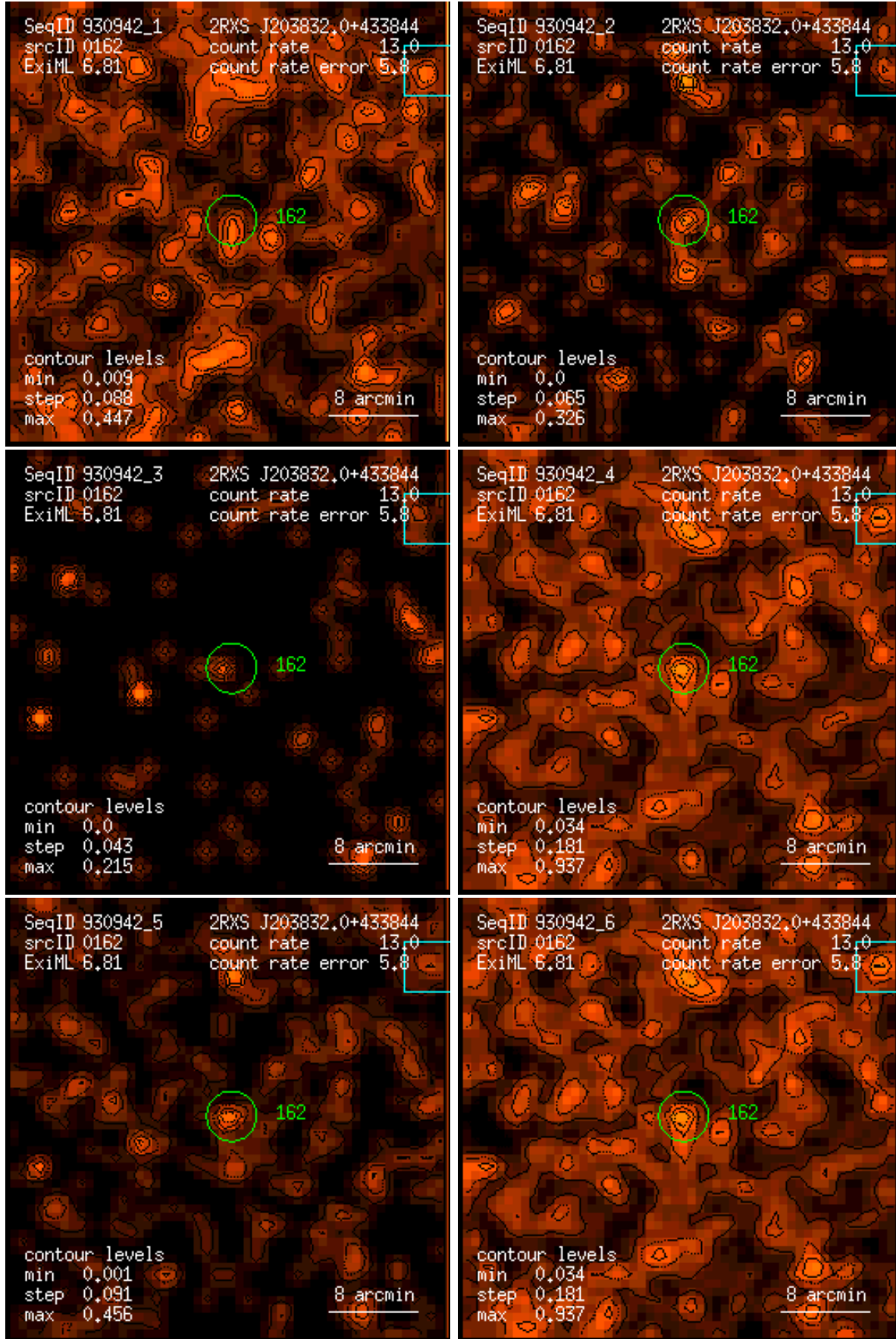
Figure 162: RASS 930942: detection 0162: band rate images, Gaussian filter: (1) PSPC channels 11 – 41, (2) 52 – 90, (3) 91 – 201, (4) 11 – 235, (5) 52 – 201, (6) 11 – 201. Broad band rates in counts/ks. Band rate contour levels in counts/ks/arcmin 2 .
