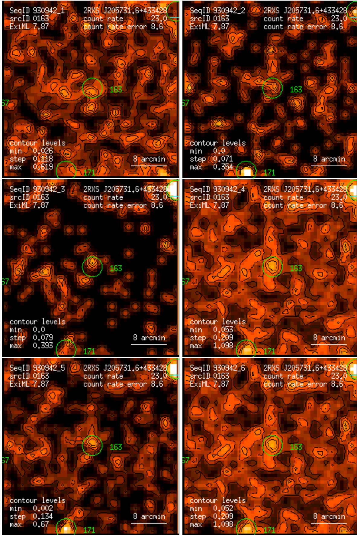
Figure 163: RASS 930942: detection 0163: band rate images, Gaussian filter: (1) PSPC channels 11 – 41, (2) 52 – 90, (3) 91 – 201, (4) 11 – 235, (5) 52 – 201, (6) 11 – 201. Broad band rates in counts/ks. Band rate contour levels in counts/ks/arcmin 2 .
