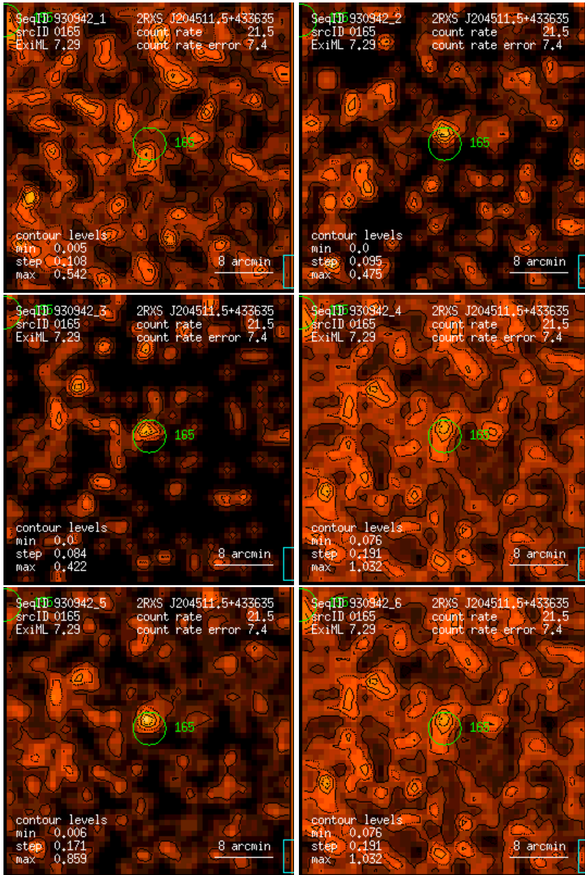
Figure 165: RASS 930942: detection 0165: band rate images, Gaussian filter: (1) PSPC channels 11 – 41, (2) 52 – 90, (3) 91 – 201, (4) 11 – 235, (5) 52 – 201, (6) 11 – 201. Broad band rates in counts/ks. Band rate contour levels in counts/ks/arcmin 2 .
