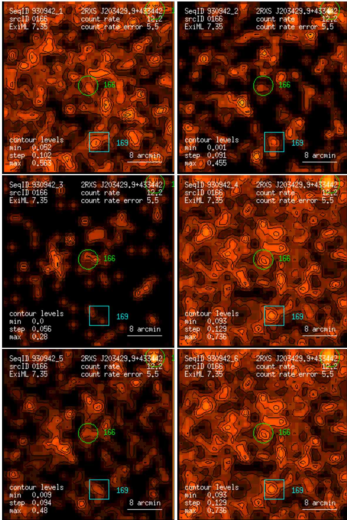
Figure 166: RASS 930942: detection 0166: band rate images, Gaussian filter: (1) PSPC channels 11 – 41, (2) 52 – 90, (3) 91 – 201, (4) 11 – 235, (5) 52 – 201, (6) 11 – 201. Broad band rates in counts/ks. Band rate contour levels in counts/ks/arcmin 2 .
